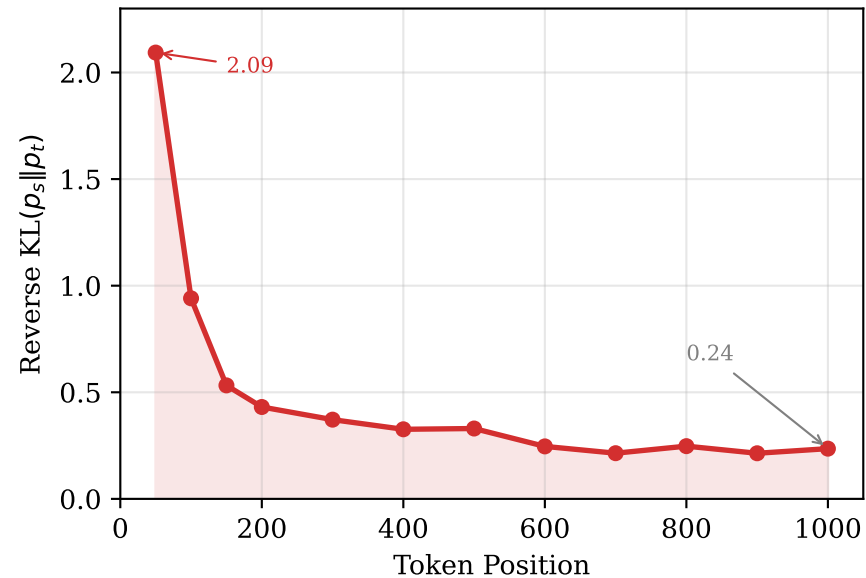
(a) Reverse KL Divergence by Position
