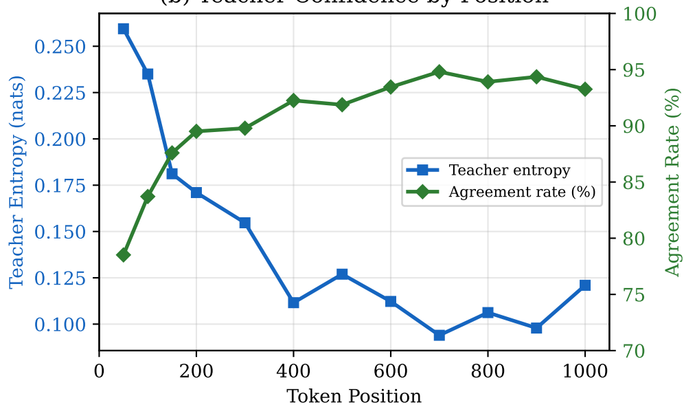
(b) Teacher Confidence by Position
