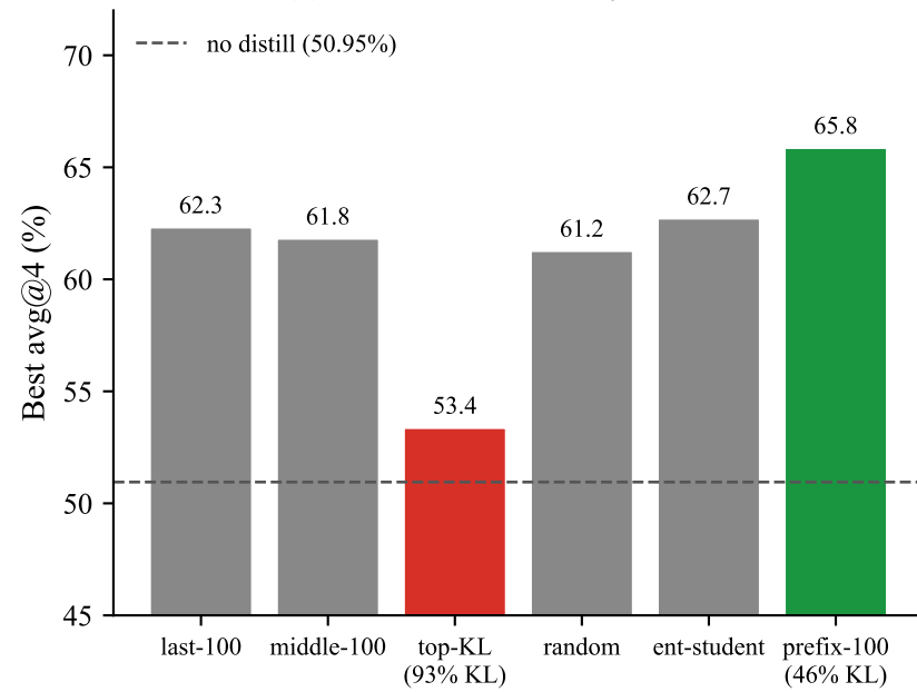
(a) Information–Quality Paradox
