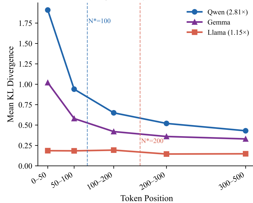
(b) Signal Decay Across Families
