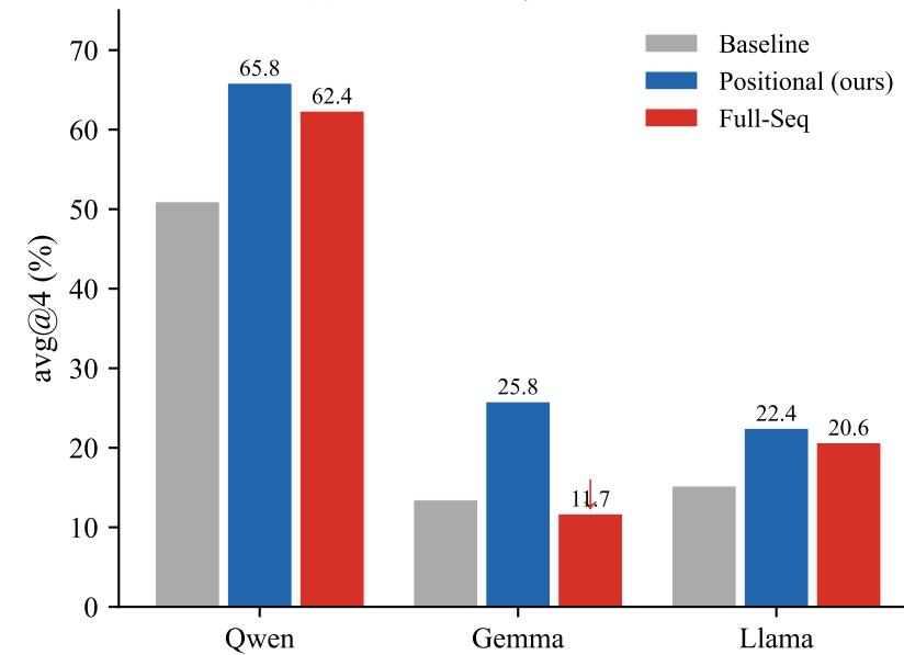
(c) Cross-Family Math Results
