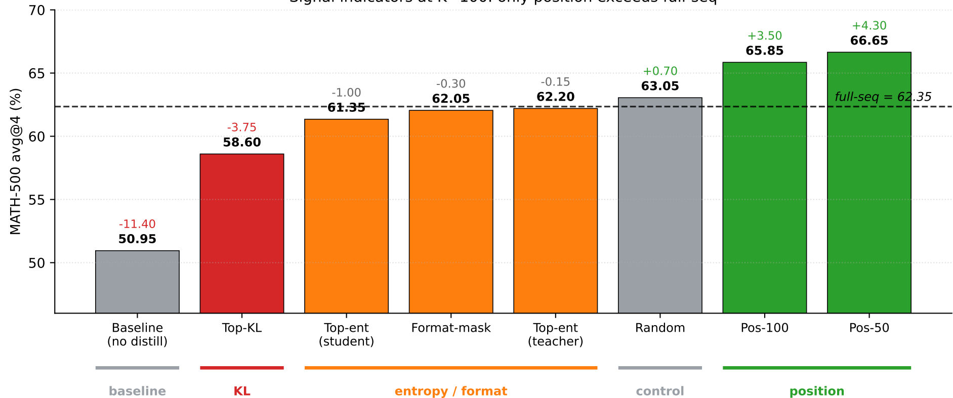
Signal indicators at K=100: only position exceeds full-seq
