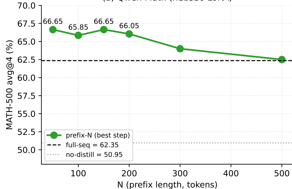
(a) Qwen Math (n1bs16 LoRA)
