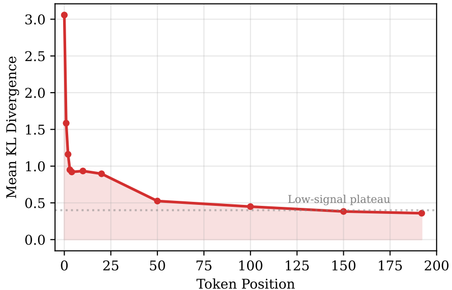
(a) KL Divergence by Position
