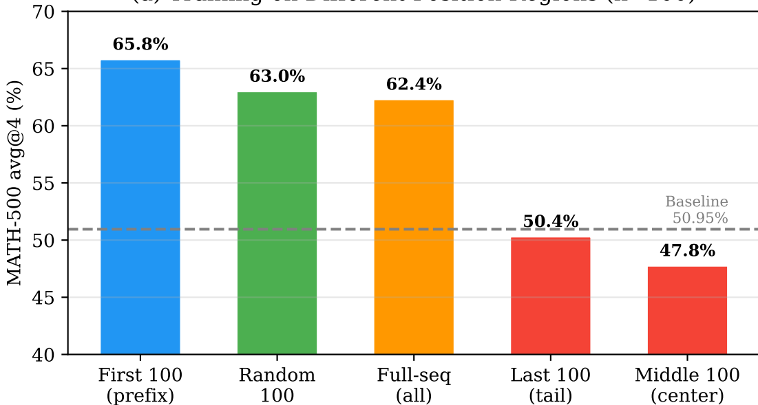
(a) Training on Different Position Regions (k=100)
