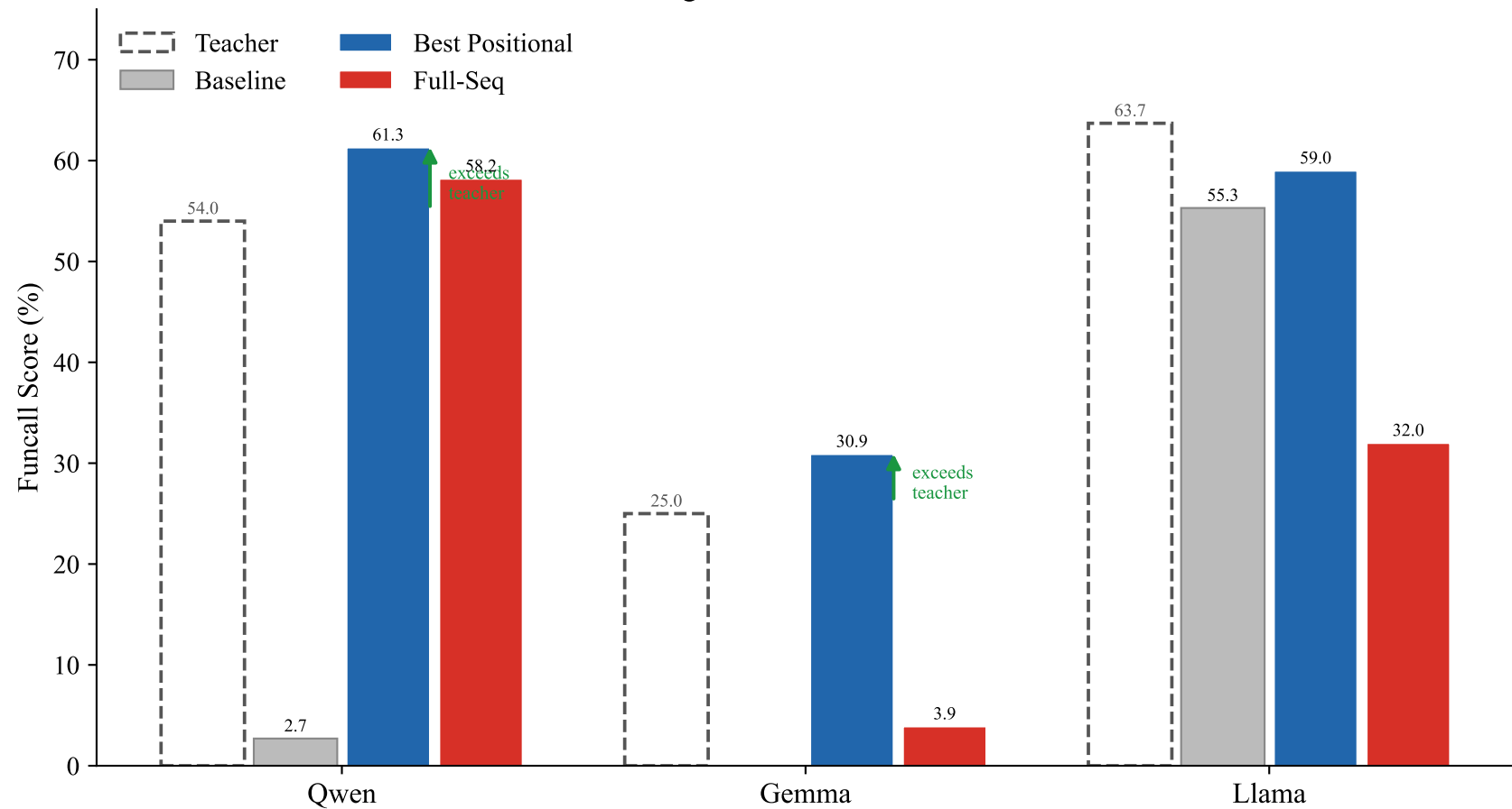
Function-Calling: Student vs. Teacher Performance
