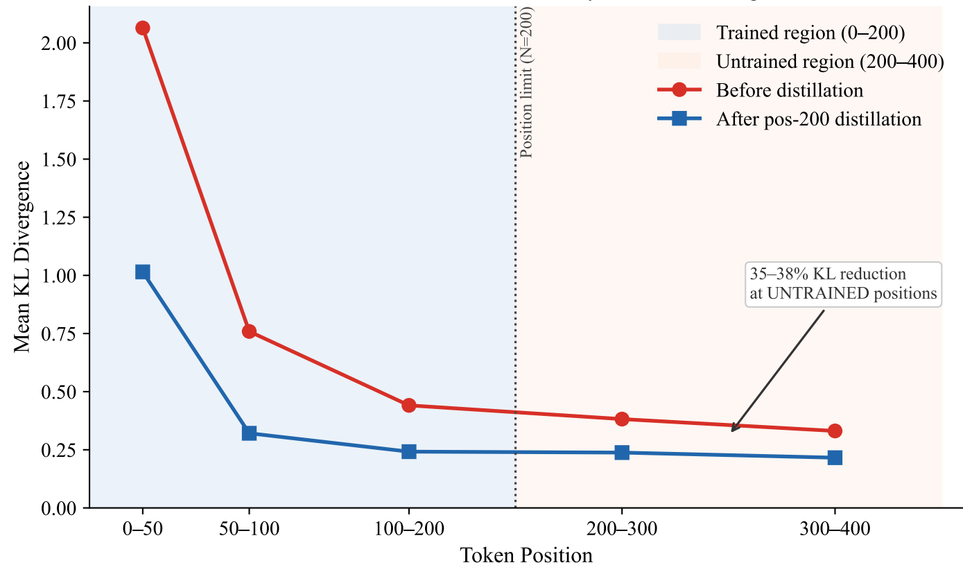
Cascade Effect: KL Reduction Beyond Trained Region
