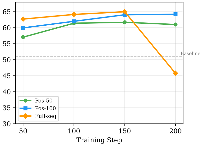
(b) 4B Teacher — Math
