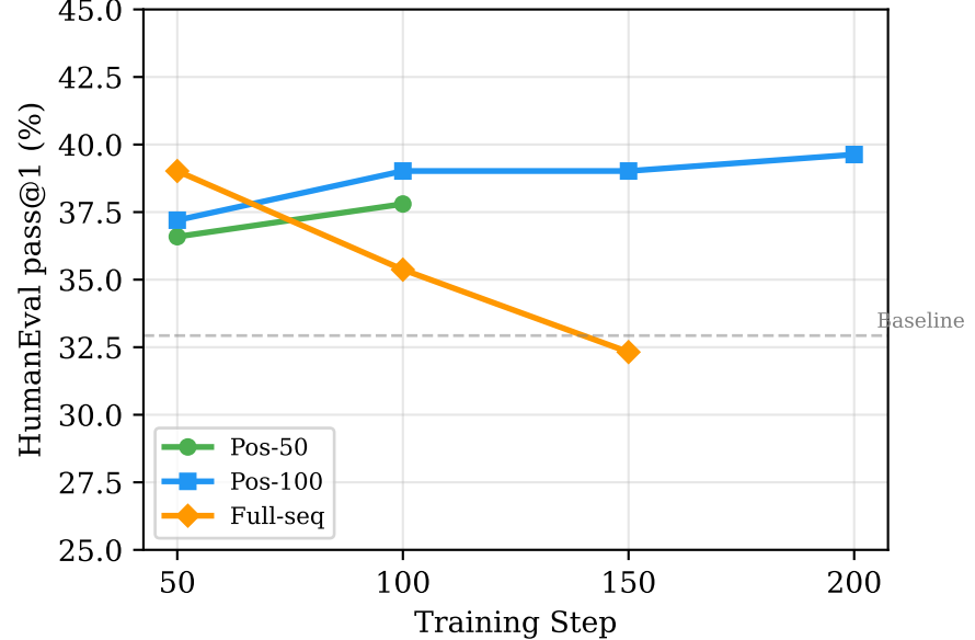
(c) 1.7B Teacher — Coding
