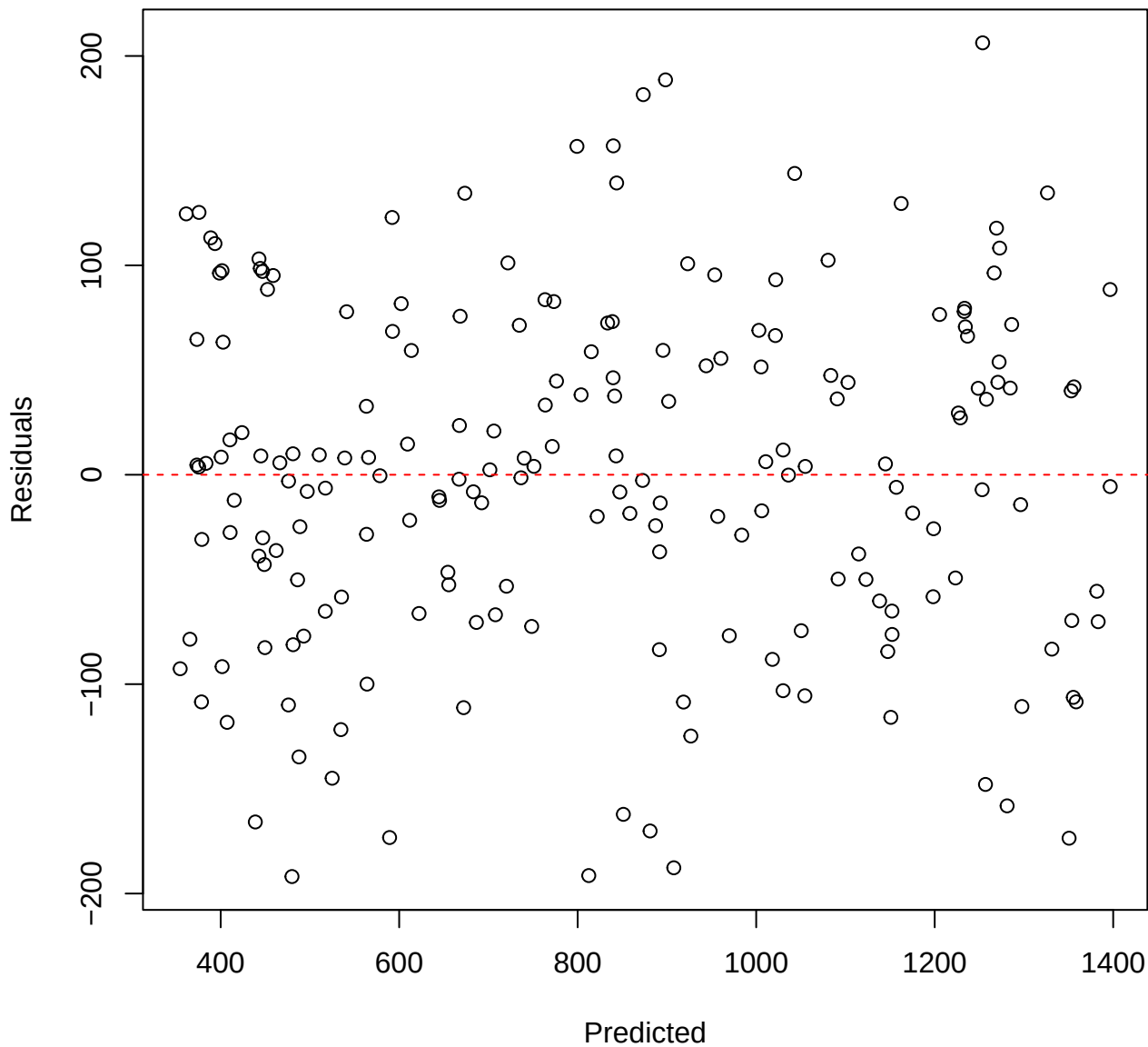
Residual Plot
