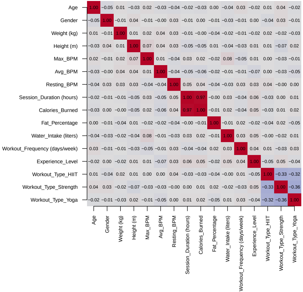
Correlation Heatmap
