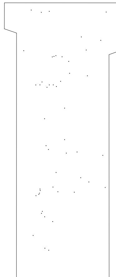
Drill Map: • 0.300mm / 0.0118" (50 holes)
