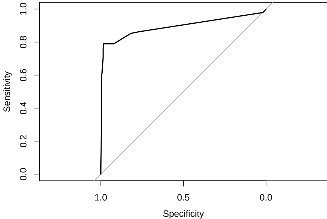
Figure 11. ROC Curve for Decision Tree
