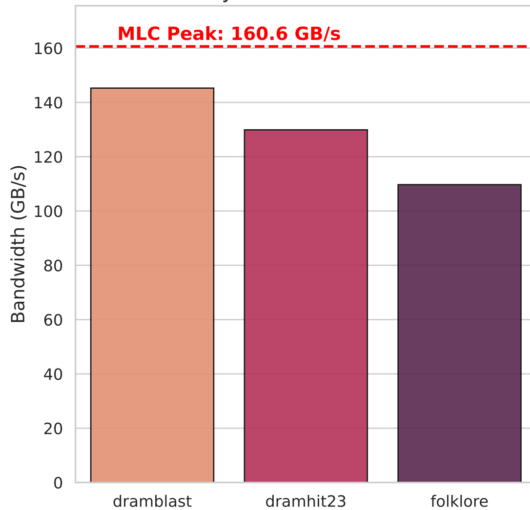
Memory Bandwidth Utilization
