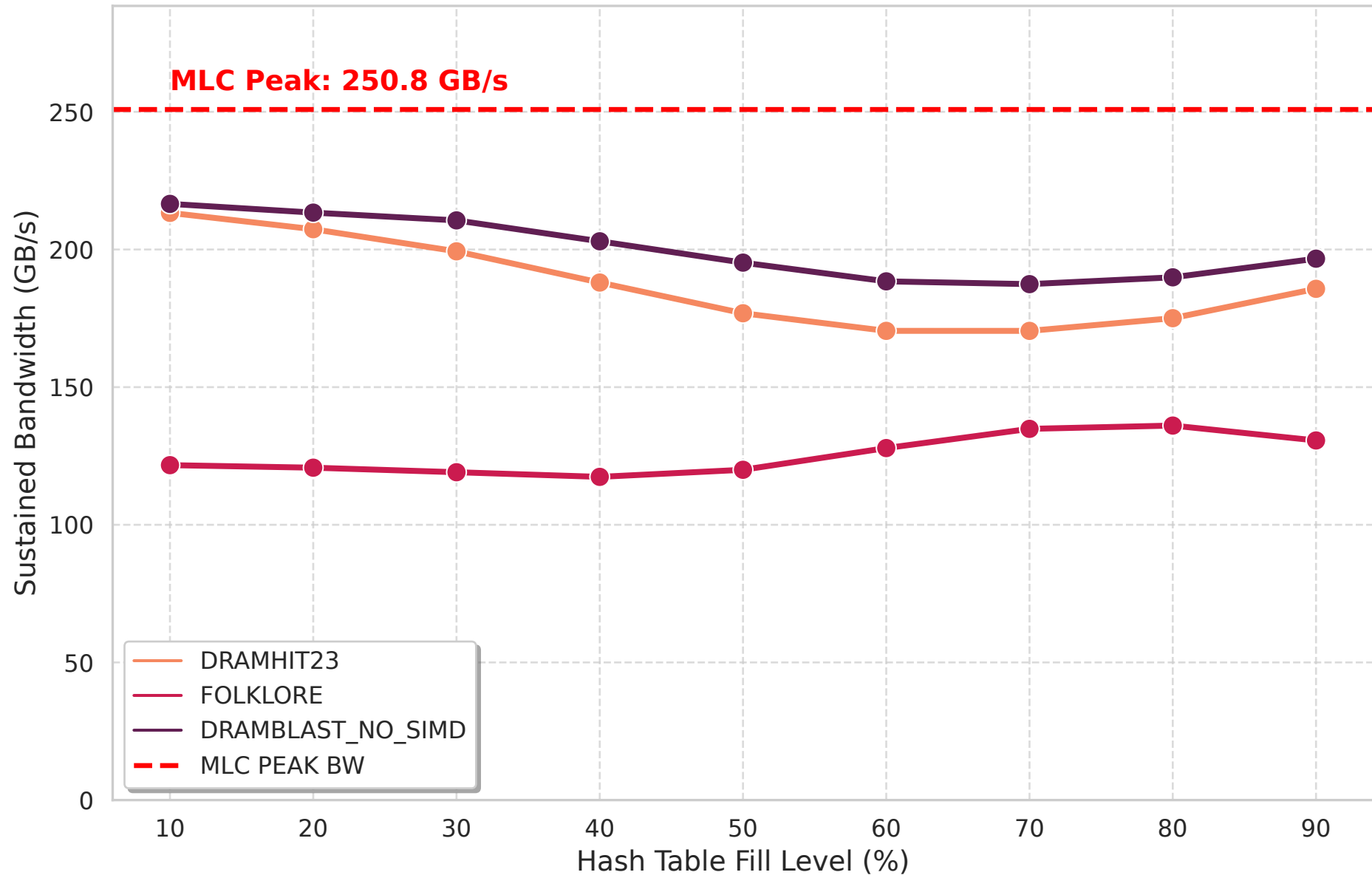
Memory Bandwidth Scaling vs. Table Fill Factor
