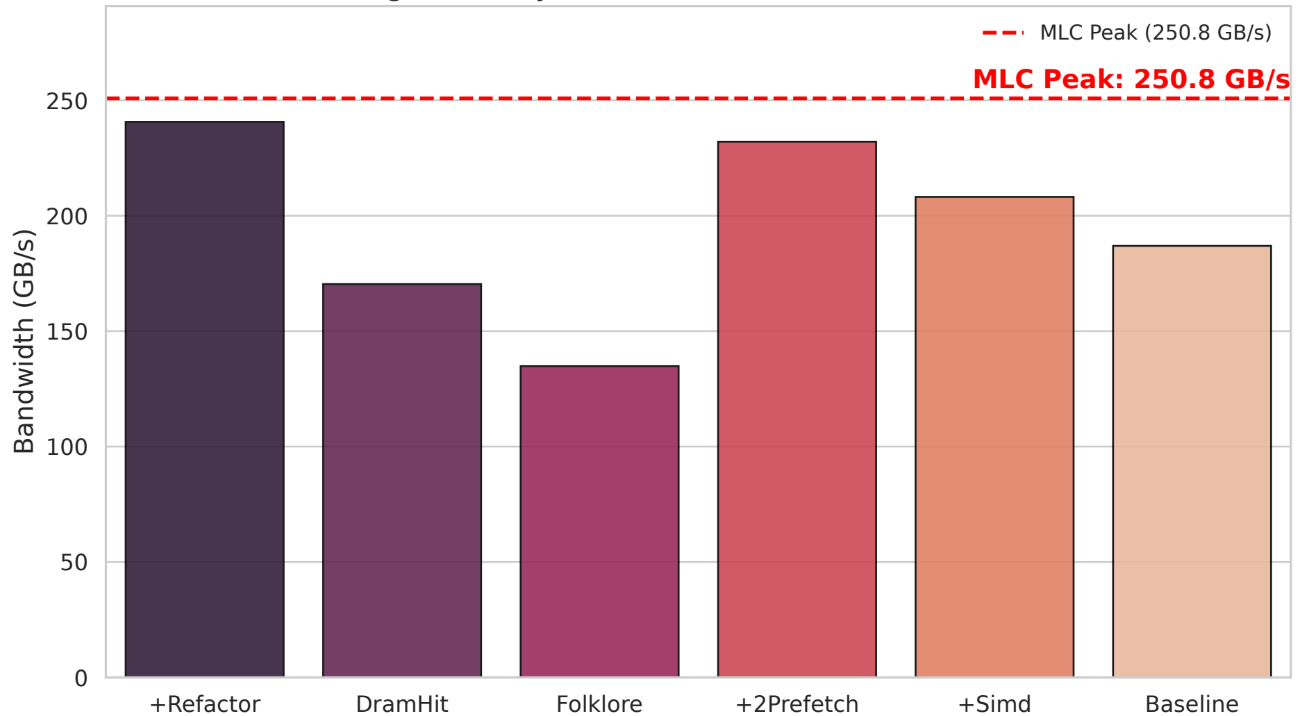
Average Memory Bandwidth (70% Fill, Find Workload)
