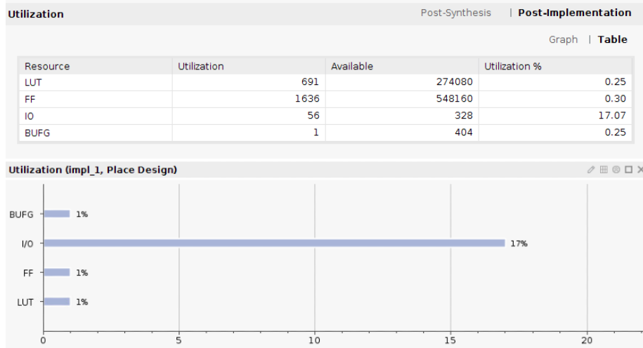
Figure 14: The resource statistics for the pedestal subtraction algorithm generated from HLS with an SSR mechanism built into the design, to be compared to the original PedSub_SSR block written directly in VHDL.
