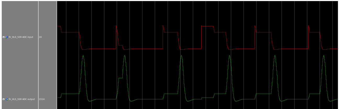
Figure 16: The analogue waveforms of ADC input and output signals generated in a Questasim simulation. This is not to scale; the green peaks are amplified to much larger values than the red peaks in true scale, reducing the likelihood of false hit readings. Random signal noise is also reduced. Plateaus in the ADC values are a result of the random back pressure events pausing block operation.
