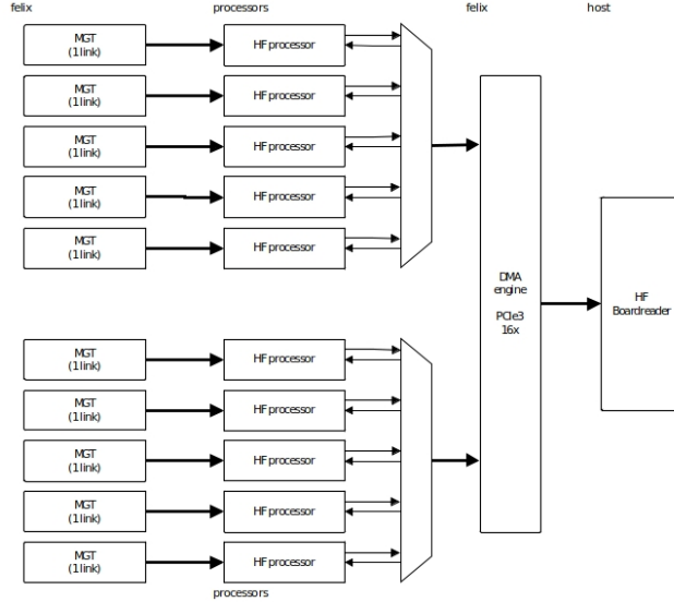
Figure 2: Overview of the Felix architecture in ProtoDUNE [29]
