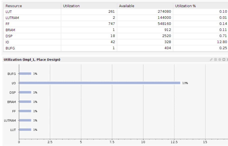
Figure 21: The resource statistics for the previously built FIR algorithm with the SSR mechanism included in the usage. This is included to allow the comparison to the HLS FIR block with an in-built SSR mechanism.
