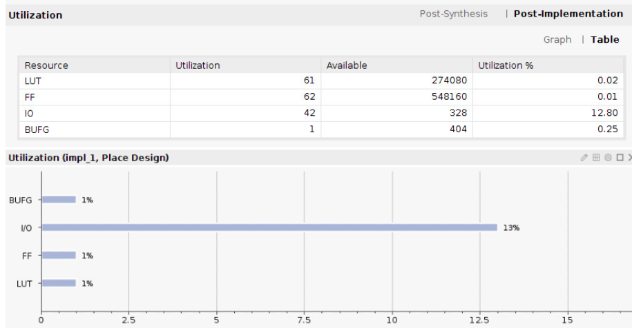
Figure 12: The resource utilisation for the original pedestal subtraction block including the exact figures above and percentage utilization below. All resource statistics were taken from the Vivado Project Manager post-implementation report summary, generated for each block. Please note that for all resource bar charts, utilization percentages above 1% have been rounded to the nearest percent. Utilizations below 1% are rounded up to the nearest percent.
