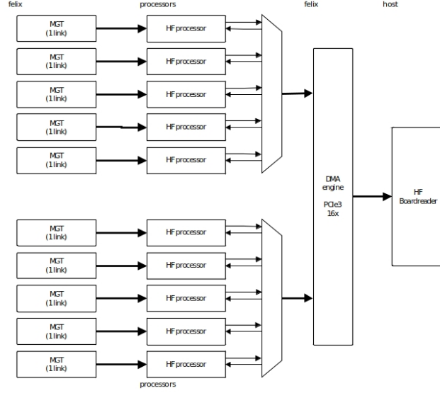
Figure 7: Overview of the FELIX architecture in ProtoDUNE II [46]. 10 MGT links turn optical data into computational bits, which then are fed into the same number of HF processors to detect and record hit packets. The resulting outputs are multiplexed into the CR, processed and finally sent to the back-end DAQ system.
