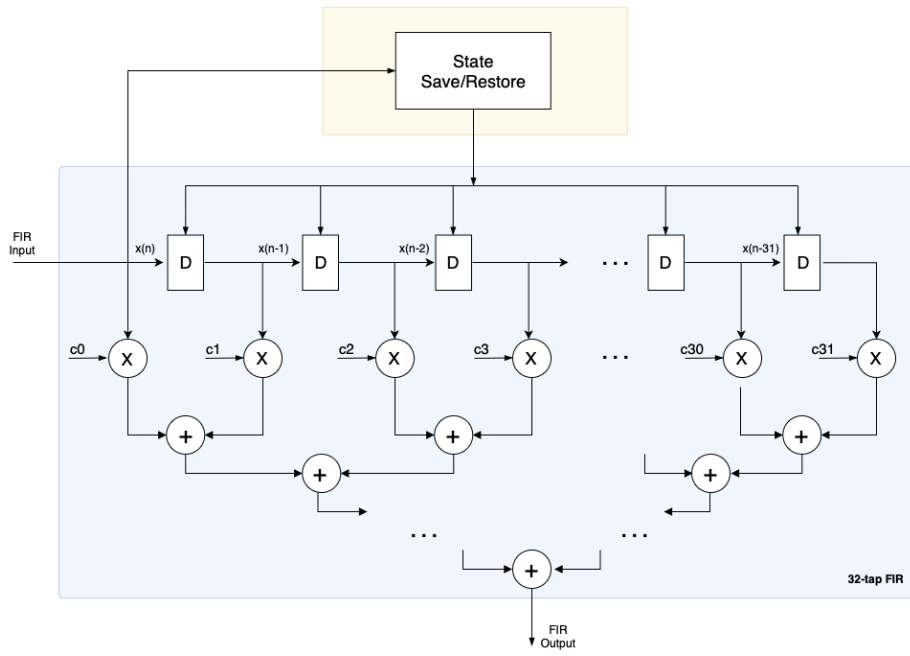
Figure 18: A visualisation of the FIR filter's manipulation of incoming ADC values, including the register shift, coefficient multiplication, sum tree and the saving and restoring of the final 32 tap values [46].
