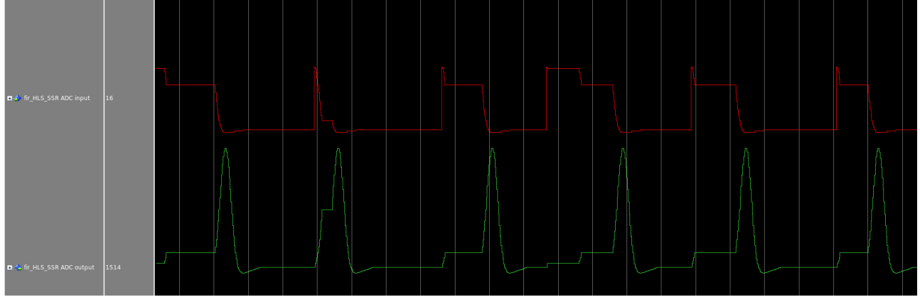
Figure 17: The analogue waveforms of ADC input and output signals generated in a Questasim simulation. This is not to scale; the green peaks are amplified to much larger values than the red peaks in true scale, reducing the likelihood of false hit readings. Random signal noise is also reduced. Plateaus in the ADC values are a result of the random back pressure events pausing block operation.
