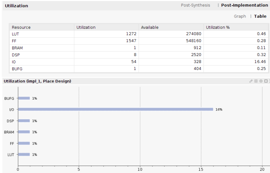
Figure 22: The resource statistics for the HLS-synthesized FIR algorithm with an in-built SSR memory and access mechanism. This enables a comparison to the manual HDL version.
