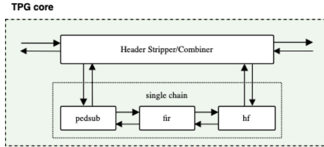
Figure 9: Focus on the TPG core and the sub-block chain, the purpose of which is to filter noise and identify hits from formatted packets received via the data router. [46].
