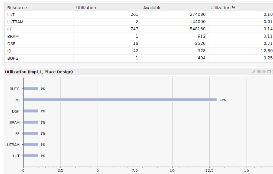
Figure 15: This figure shows the resource statistics for the previously built FIR algorithm with the SSR mechanism included in the usage. This is included to allow the comparison to the HLS FIR block with an in-built SSR mechanism.
