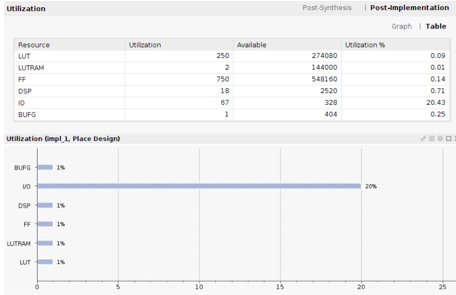
Figure 13: This figure details the resource statistics of the previously written FIR filter algorithm with the SSR mechanism not included, to allow for comparison to the analogous redesigned HLS module.
