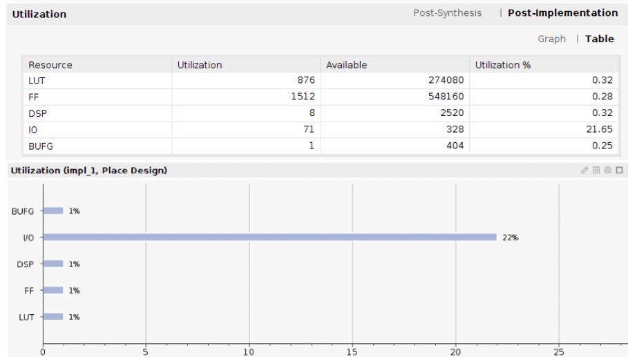
Figure 14: This figure contains the resource statistics for the FIR filter algorithm written in HLS, connected to a previously written external SSR mechanism that is not included in the statistics. The only resources being spent on the SSR are those allocated for accepting and storing the output values from the external SSR block.
