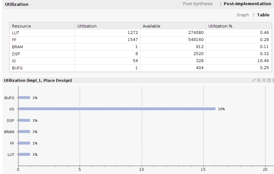
Figure 16: The above graphic demonstrates the resource statistics for the HLS-synthesized FIR algorithm with an in-built SSR memory and access mechanism, to enable the comparison to the version written from scratch in a HDL.
