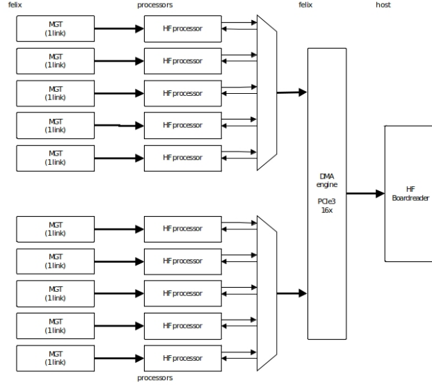
Figure 6: Overview of the FELIX architecture in ProtoDUNE II [46]. 10 MGT links turn optical data into computational bits, which then are fed into the same number of HF processors to detect and record hit packets. The resulting outputs are multiplexed into the CR, processed and finally sent to the back-end DAQ system.
