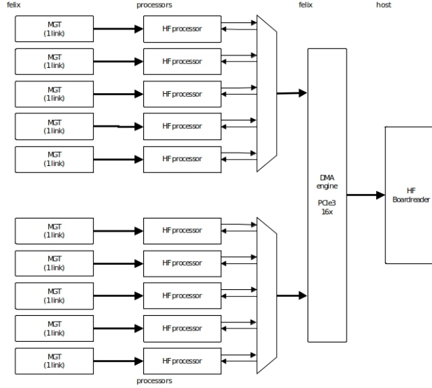
Figure 2: Overview of the Felix architecture in ProtoDUNE [34]
