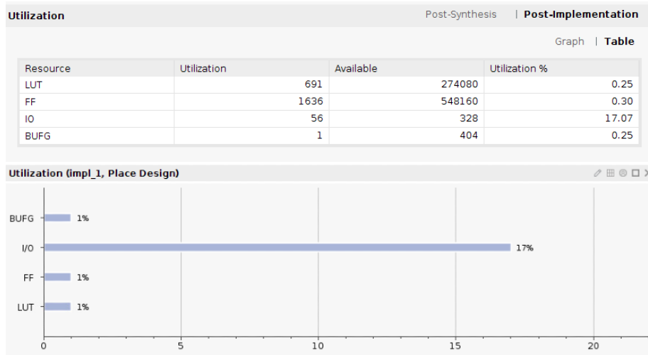
Figure 9: This figure details the resource statistics for the pedestal subtraction algorithm generated from HLS with an SSR memory built into the design.
