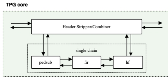
Figure 8: Focus on the TPG core and the sub-block chain [46].
