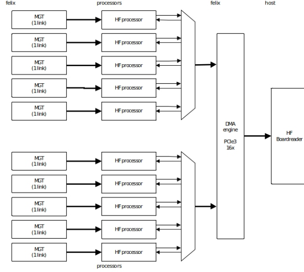
Figure 4: Overview of the Felix architecture in ProtoDUNE [38]
