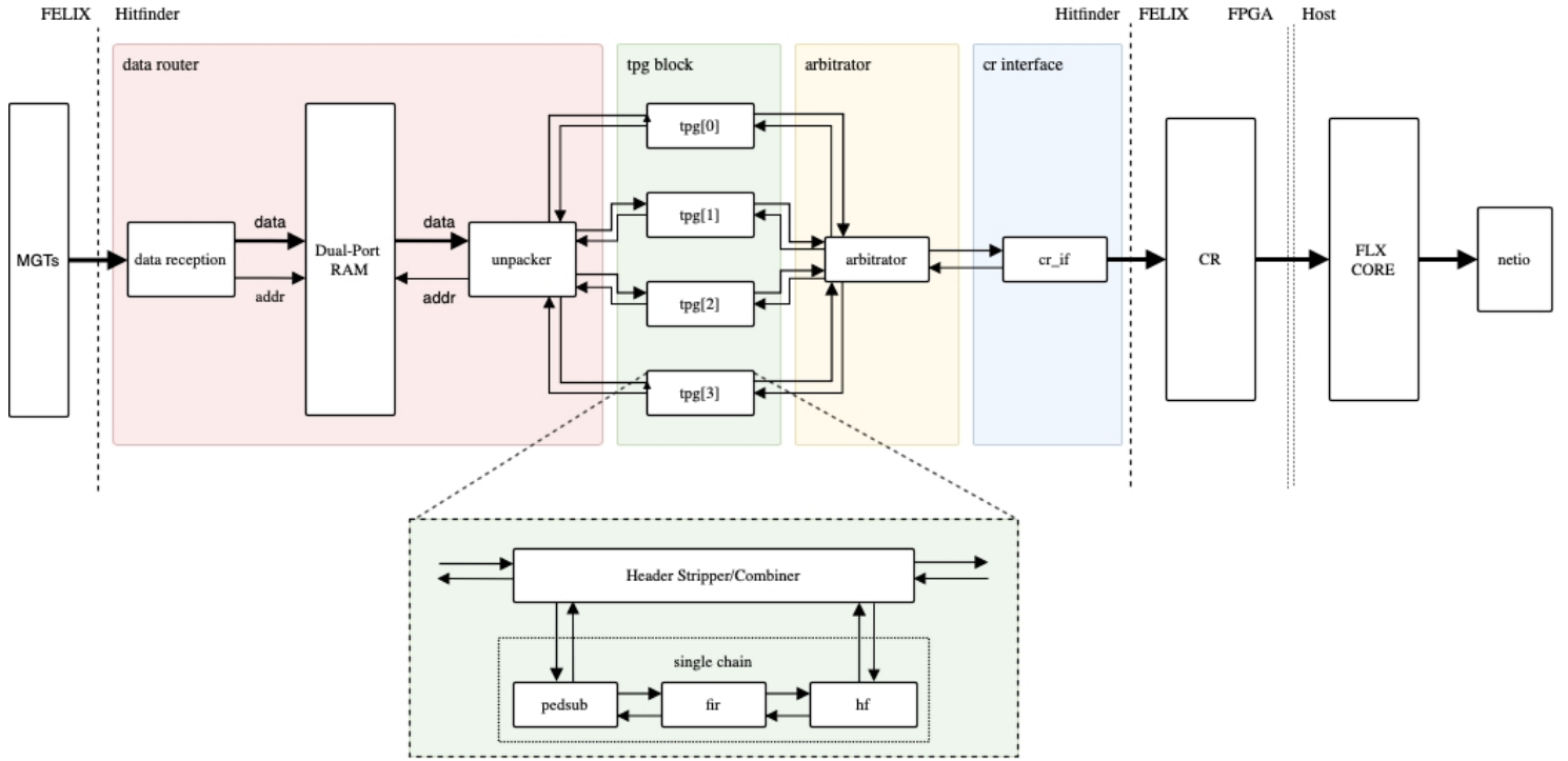
Figure 5: Hit Finder Firmware Architecture [38].
