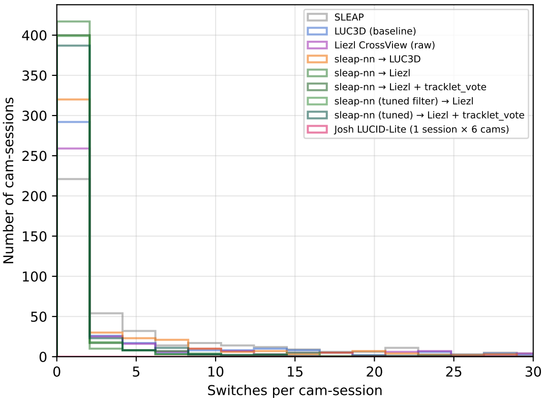
C. Per cam-session switch distribution
