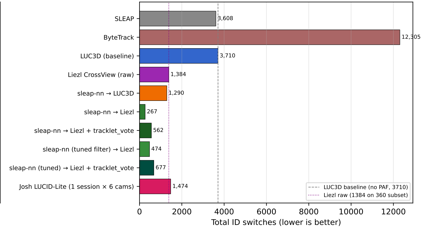
B. Total switches by tracker
