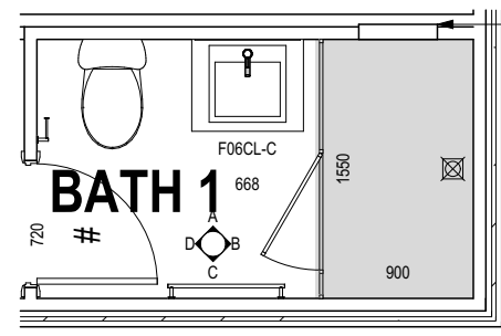
BATHROOM 1 PLAN (GRANNY FLAT) SCALE: 1:50
