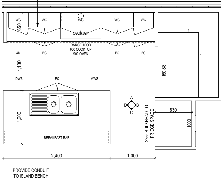
KITCHEN PLAN SCALE: 1:50
