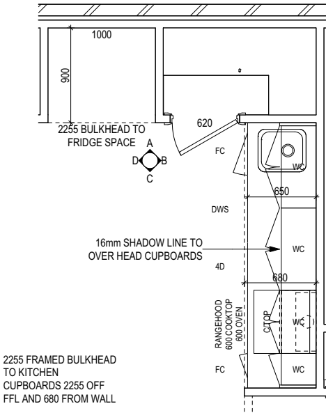
KITCHEN PLAN (GRANNY FLAT) SCALE: 1:50
