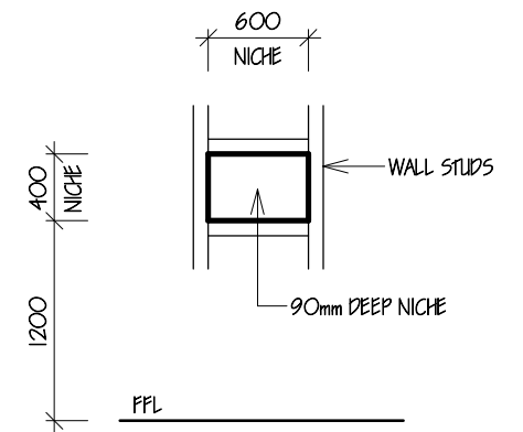
Shower Niche Detail
