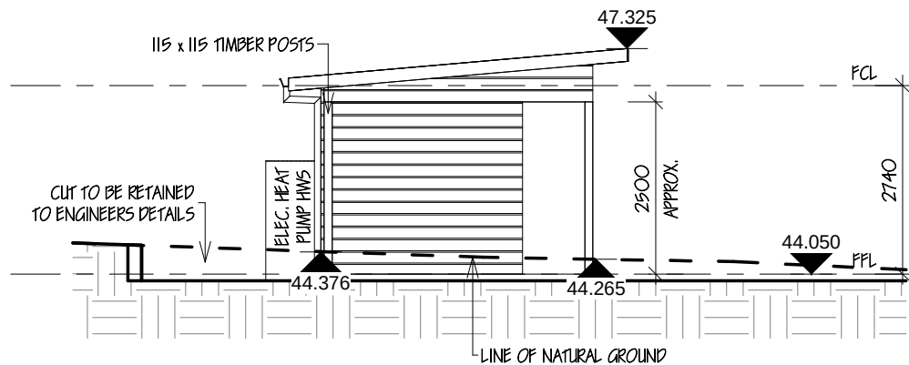
1 Cabana South Elevation 1 : 100
