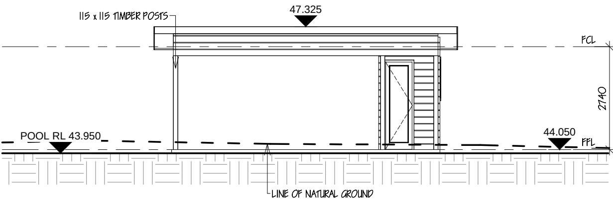
2 Cabana East Elevation 1 : 100
