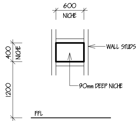
4 Shower Niche Detail 1 : 50
