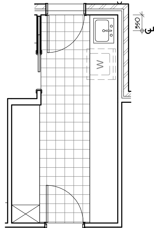
Laundry Detail
