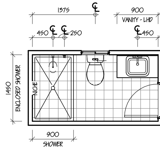
PDR Detail
