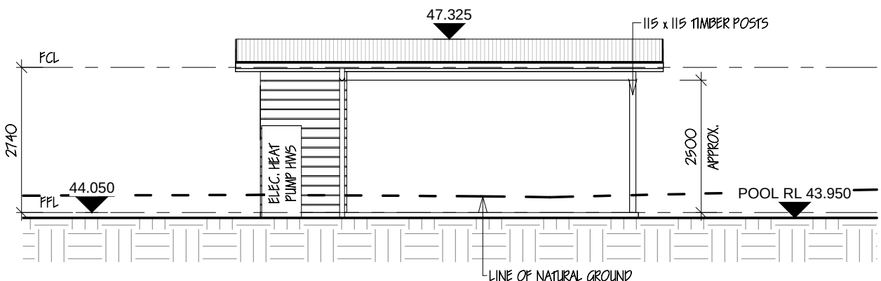
3 Cabana West Elevation 1 : 100
