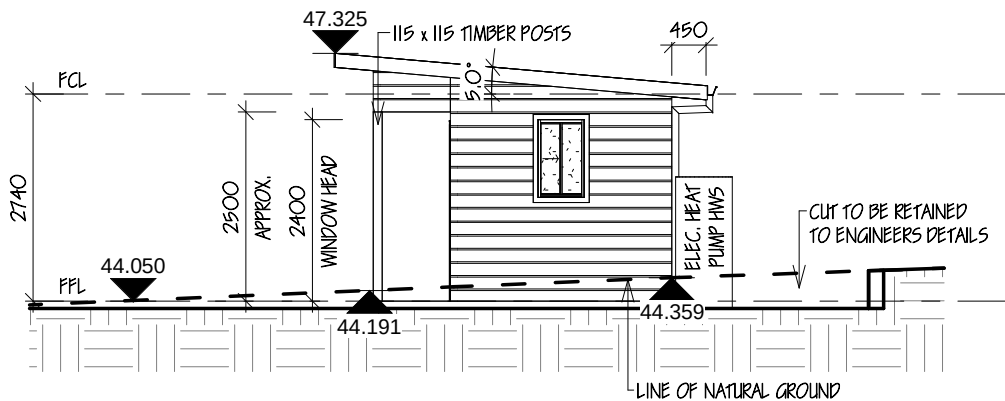
4 Cabana North Elevation 1 : 100
