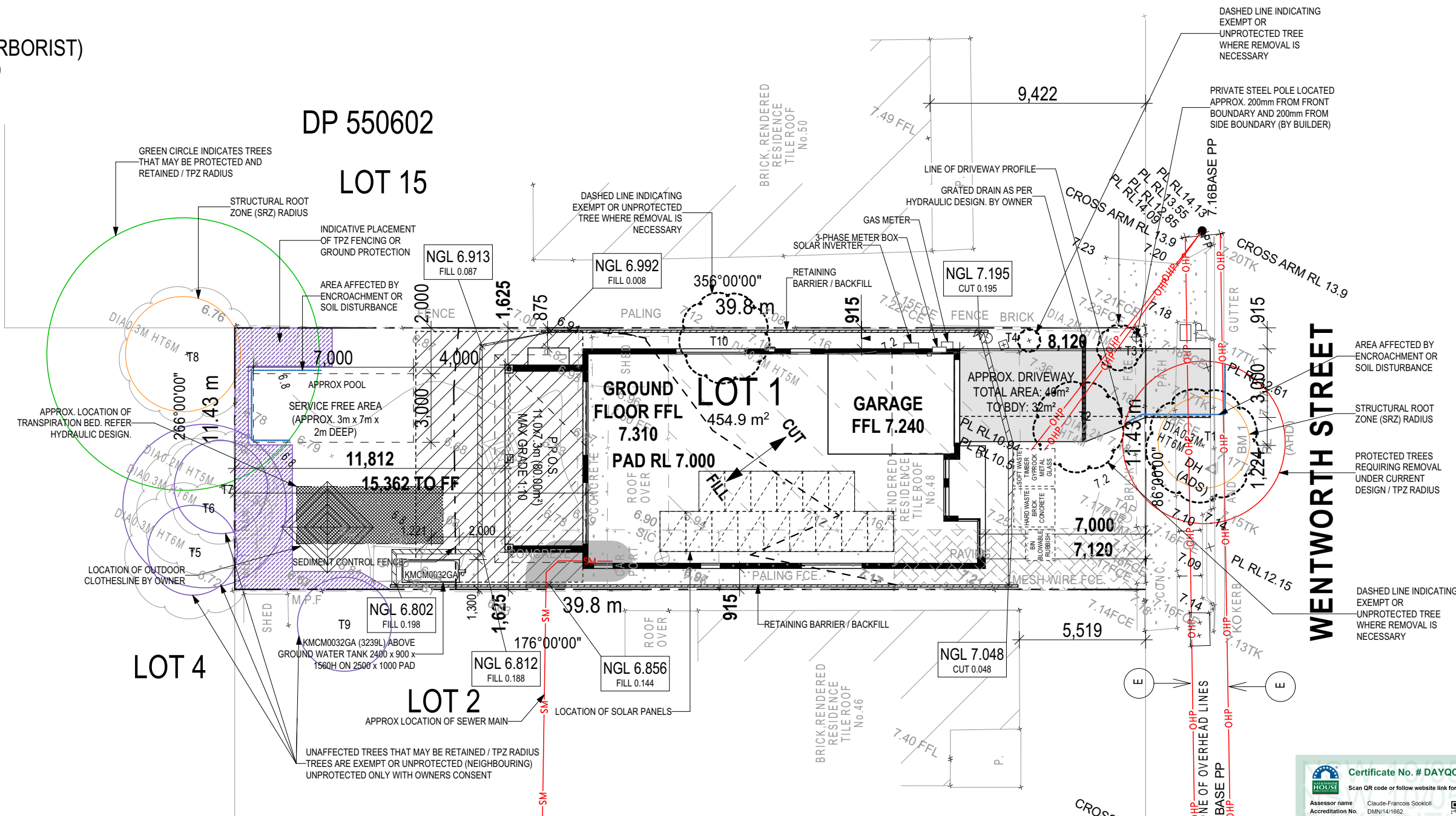
SITE PLAN (TPZ-ARBORIST) SCALE: 1:200
