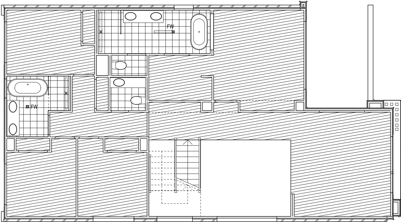
FLOOR COVERINGS (FIRST FLOOR) SCALE: 1:100
