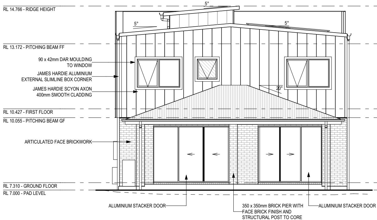
REAR ELEVATION ( SOUTH ) SCALE: 1:100
