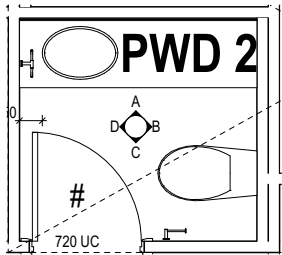
POWDER ROOM 2 PLAN SCALE: 1:50
