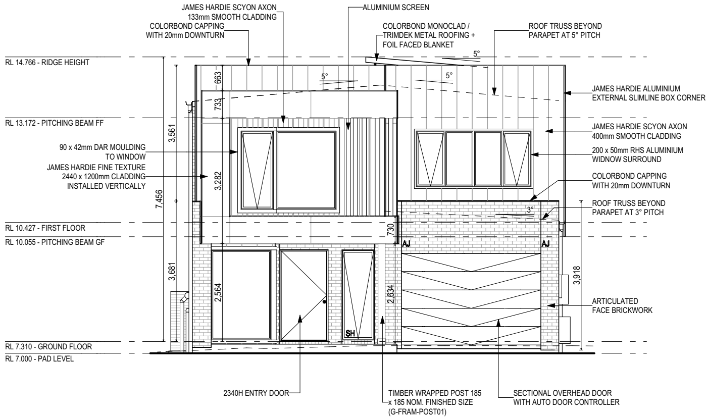
FRONT ELEVATION ( NORTH ) SCALE: 1:100
