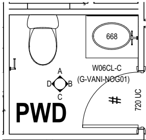
POWDER ROOM PLAN SCALE: 1:50
