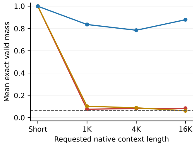
Selected checkpoint: dependent posterior, four development conditions
