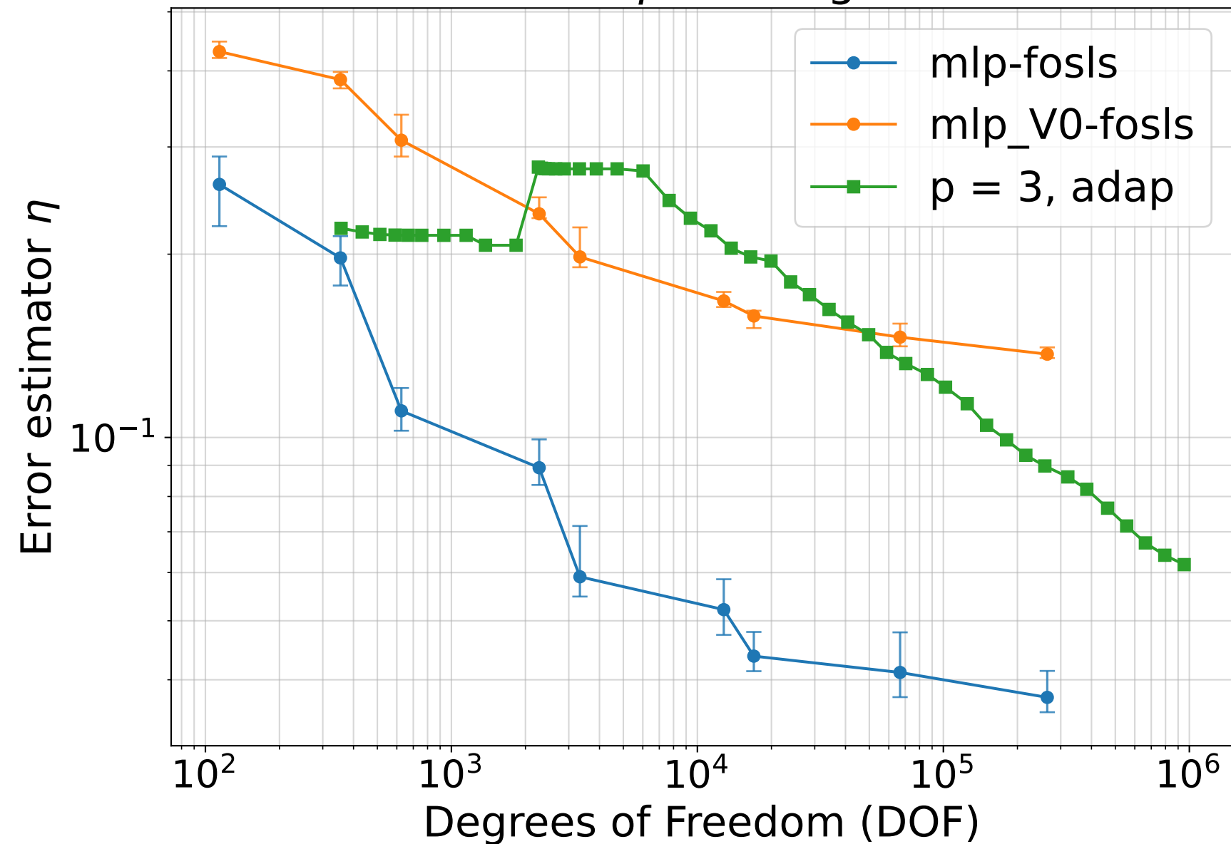
Error Estimator \eta Convergence vs DOF
