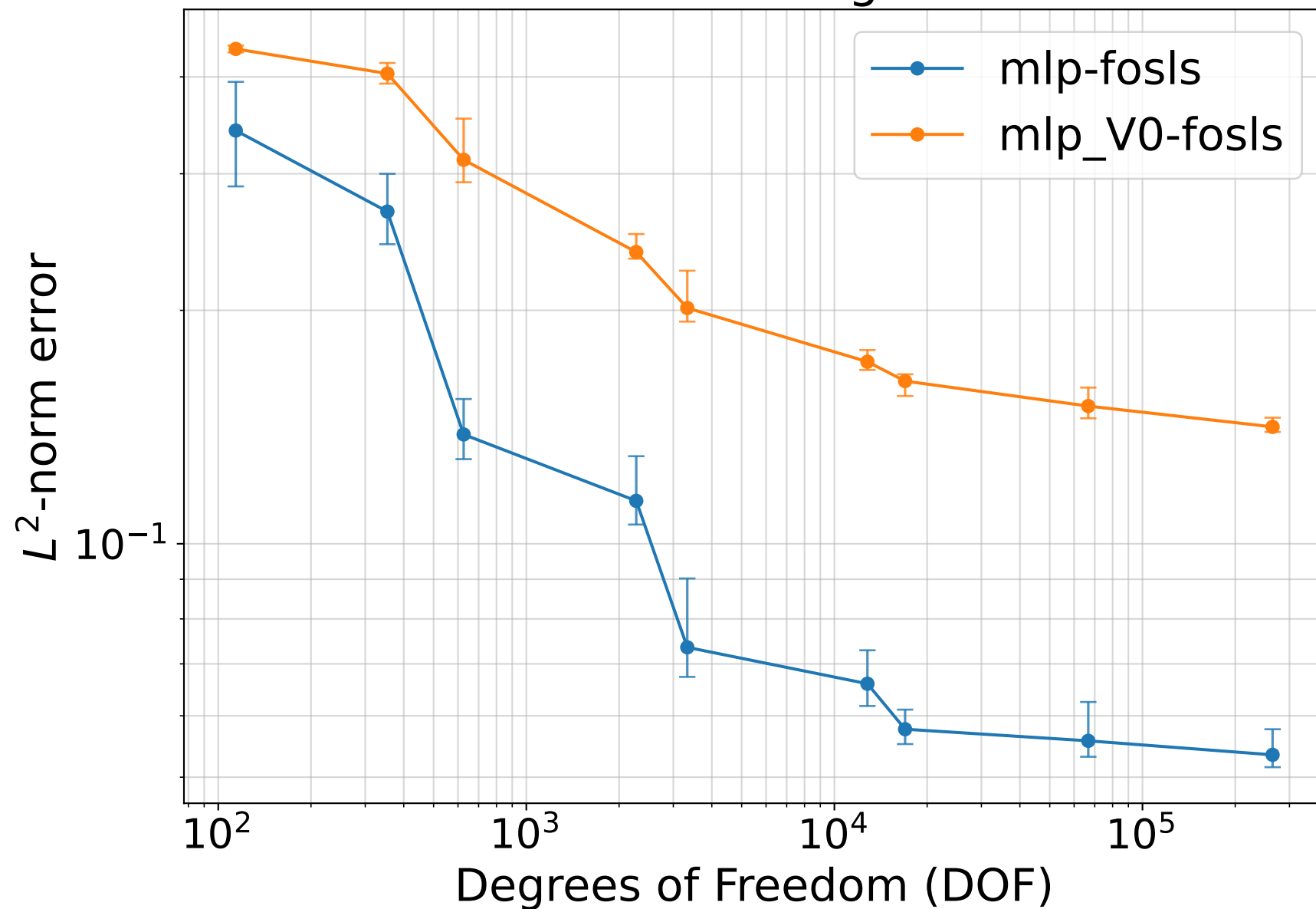
L^2 -norm Error Convergence vs DOF
