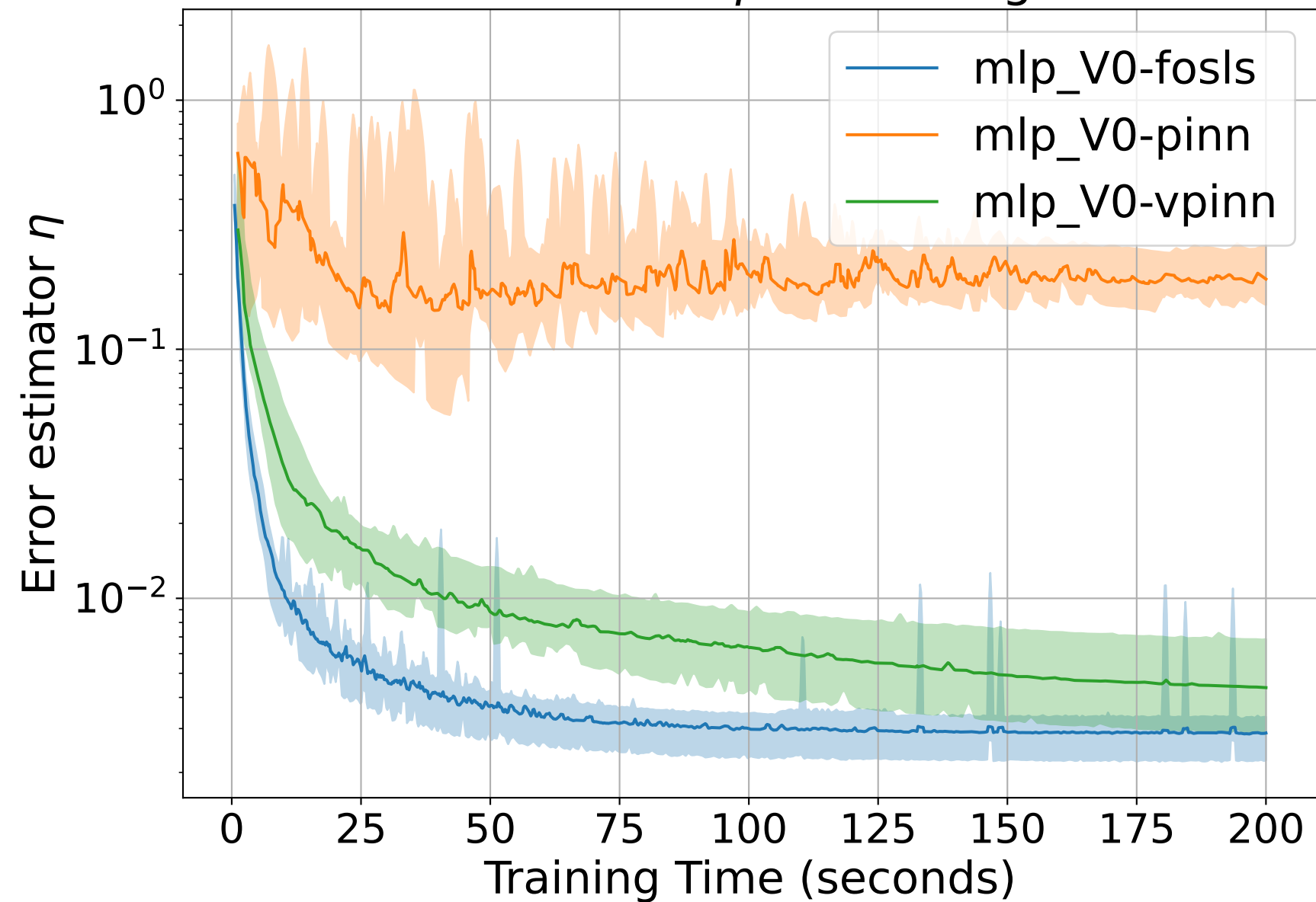
Error Estimator \eta vs Training Time
