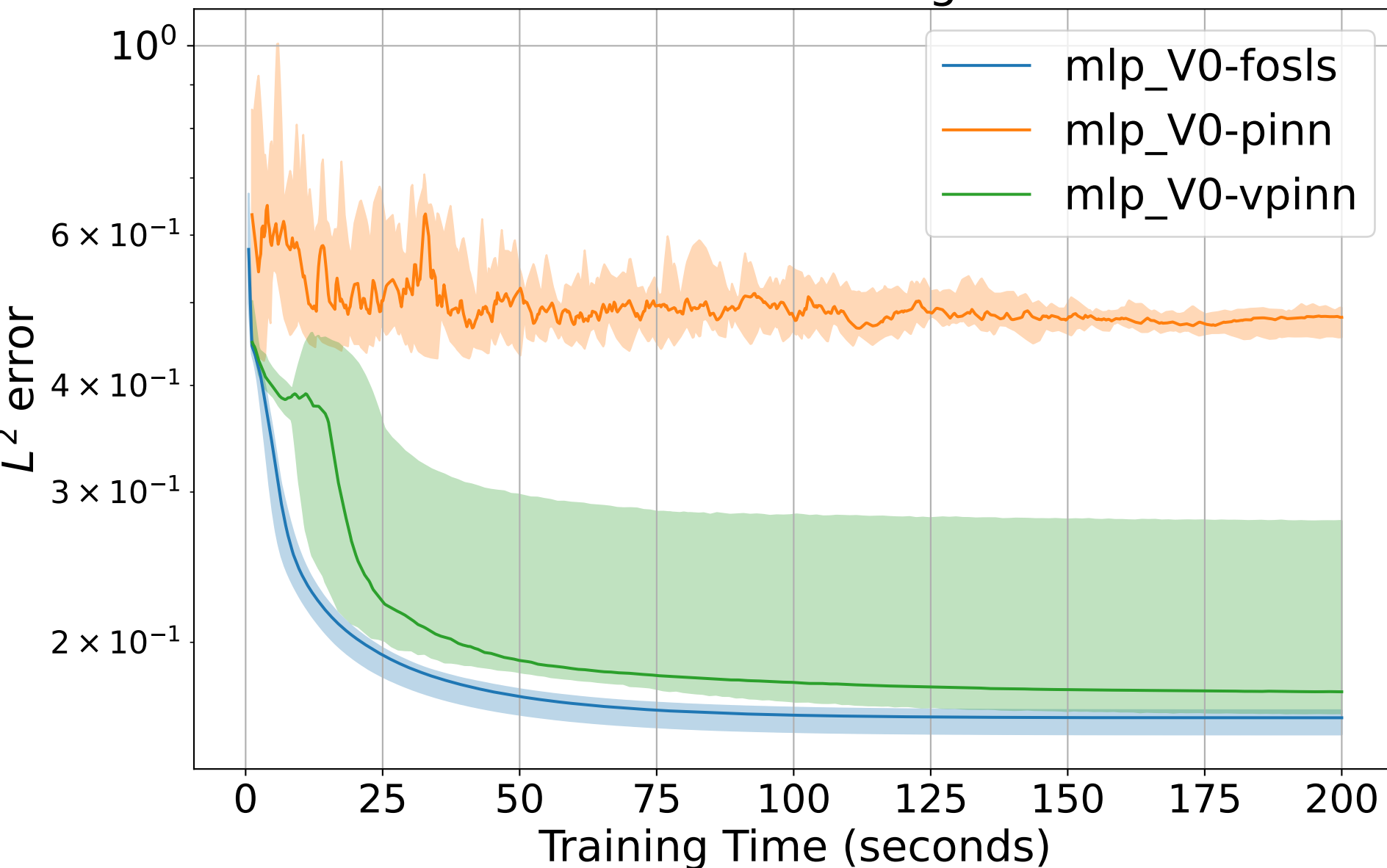
L^2 Error vs Training Time
