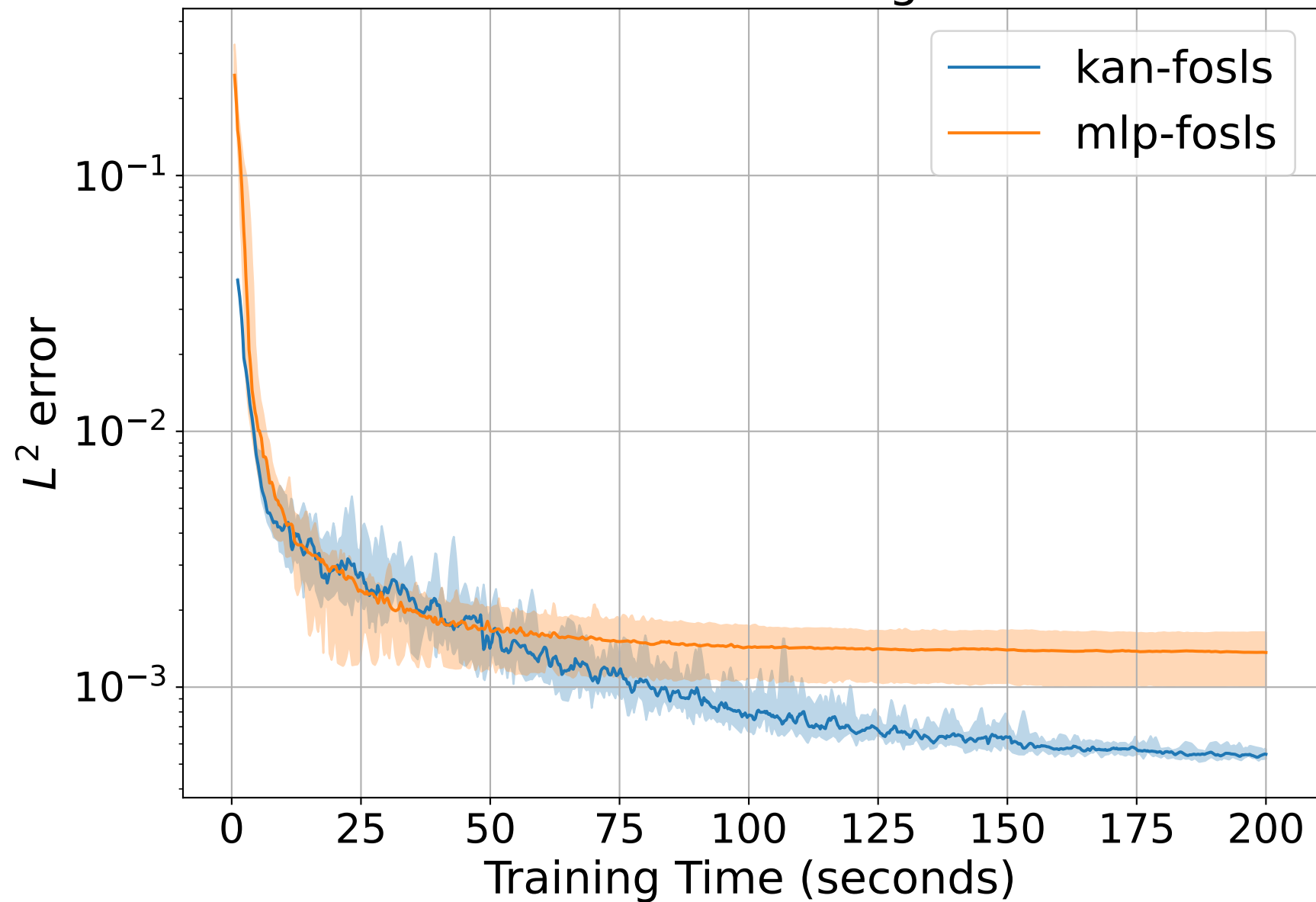
L^2 Error vs Training Time
