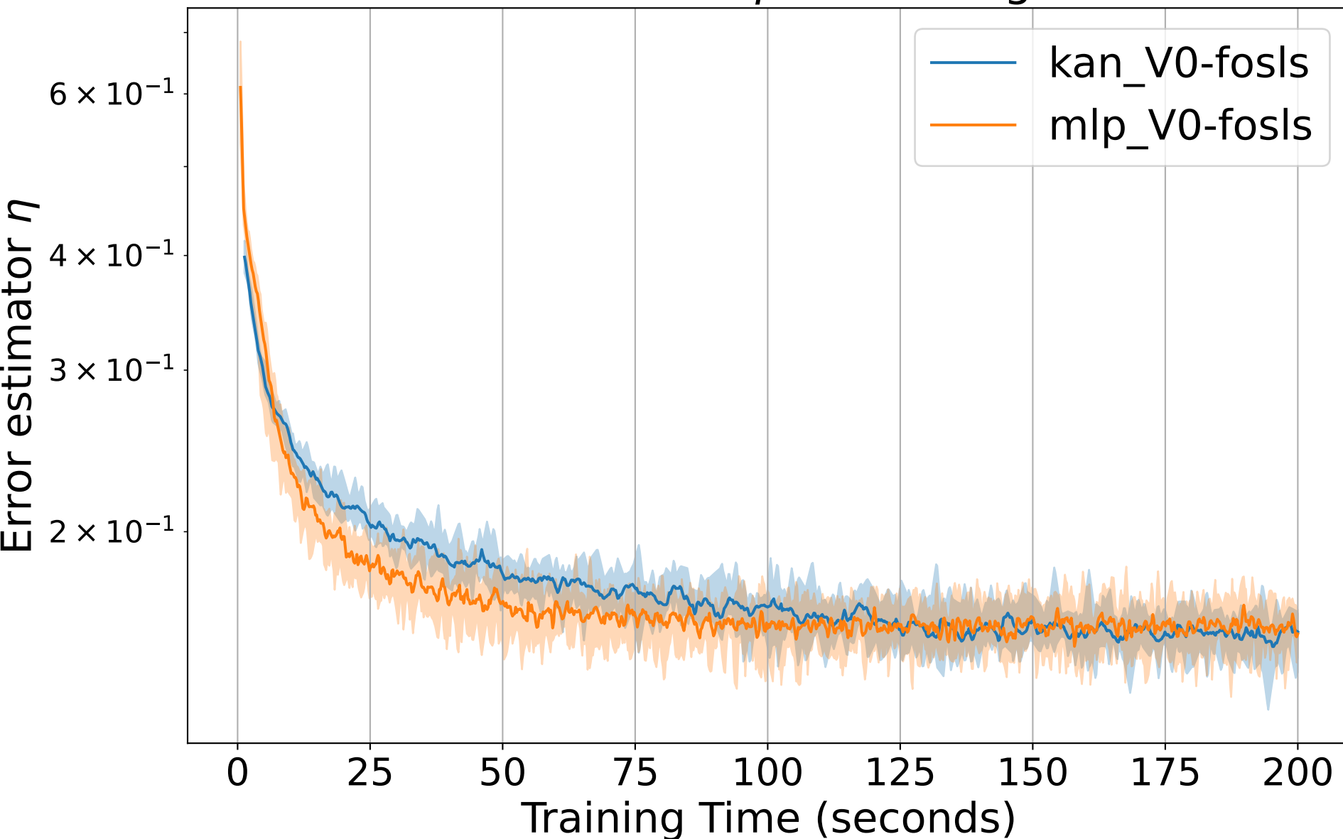
Error Estimator \eta vs Training Time
