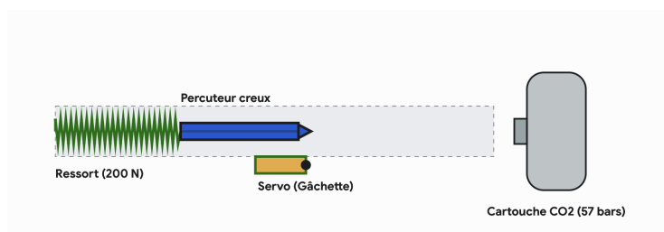
FIGURE 7 – Schéma percussion gaz
