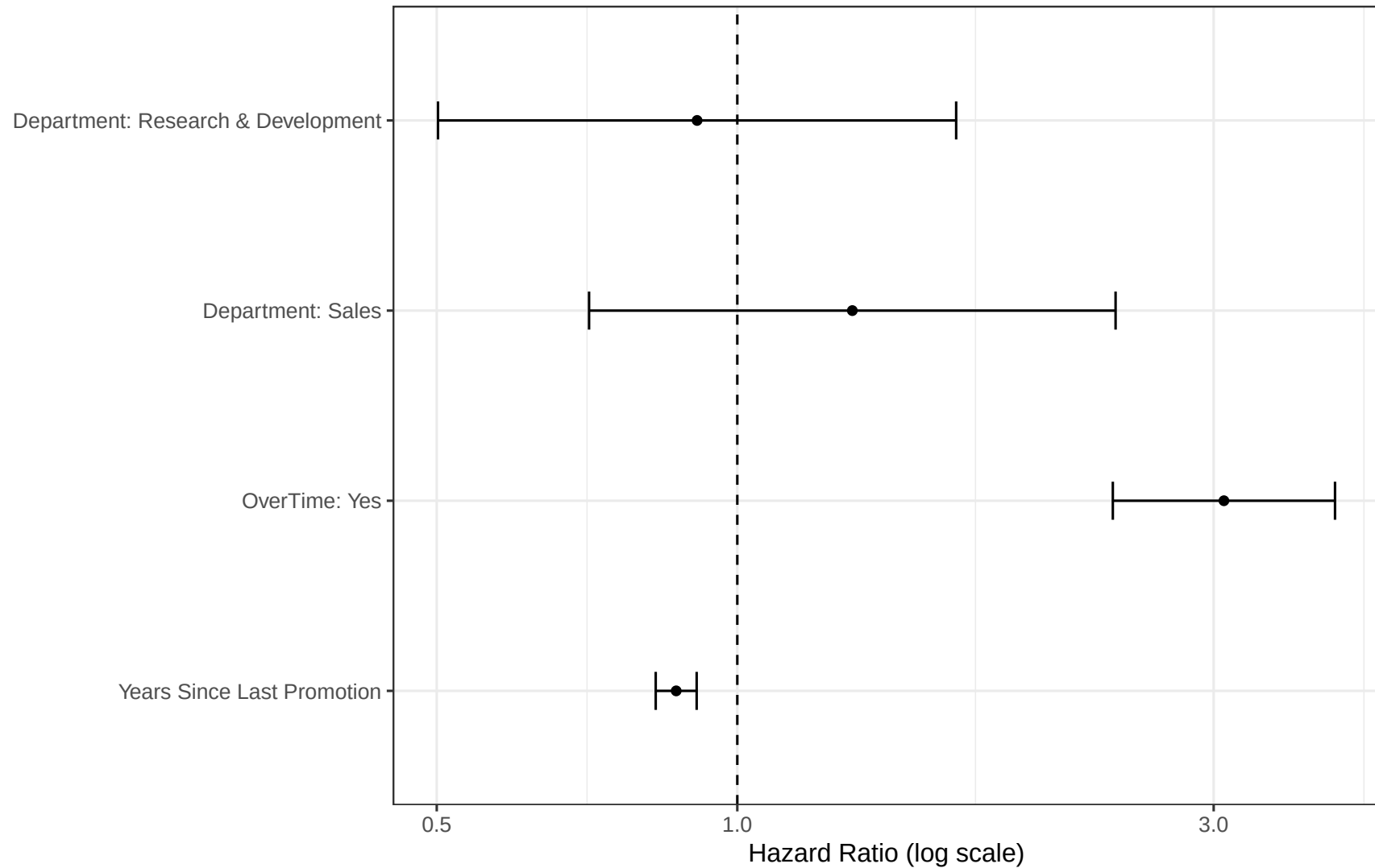
Cox Model Hazard Ratios (Attrition)
