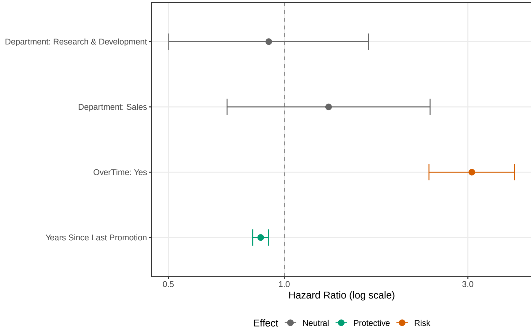
Cox Model Hazard Ratios (Attrition)
