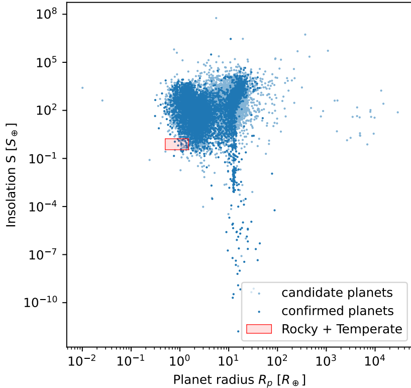
Figure 6: Distribution of the enriched Exo-MerCat exoplanet population in terms of planet-radius insolation (contains parameter computations). Confirmed planets are drawn in the darker shade and unconfirmed candidates in the lighter shade. The red rectangle marks the rocky-and-temperate selection region adopted in this work, spanning a radius of 0.5\text{--}1.5 R_{\oplus} and an incident stellar flux of 0.35\text{--}1.7 S_{\oplus} .
