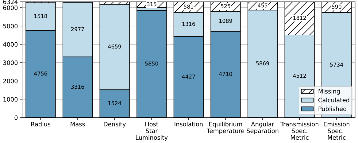
Figure 1: Provenance of pscomppars values (out of 6324 confirmed planets in total) for the nine columns in which NEA reports “Calculated Value” entries. All other columns are devoid of computations. Each bar splits the catalog into entries with a directly published measurement, entries calculated by the archive, and entries for which the parameter is missing entirely [6].
