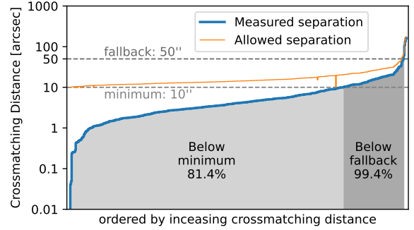
Figure 3: Calibration of coordinate crossmatching for NEA using SIMBAD IDs to crossmatch with HPICxLIFECat. The separations between matched HPICxLIFECat input stars and NEA catalog positions are plotted in increasing order and the algorithm’s 10” minimum matching tolerance and 50” fallback threshold overlaid to illustrate how the observed IDs fall within the adopted angular acceptance. The remaining 0.6% above the fallback threshold are also coordinate matched due to the proper-motion-sensitive search radius.
