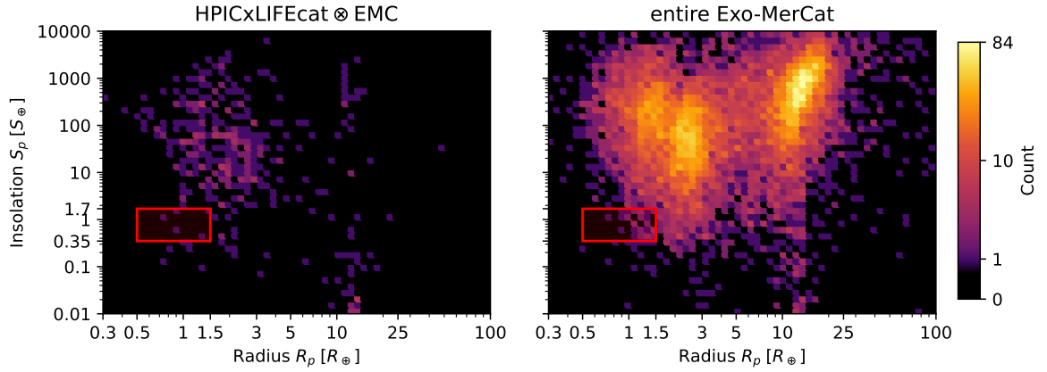
Figure 7: Two-dimensional number density heatmap of the known exoplanet population w.r.t planet-radius and insolation comparing the distributions in Exo-MerCat and Exo-MerCat matched to HPICxLIFECat. The red rectangle marks the same rocky-and-temperate selection region as in figure 6, spanning 0.5\text{--}1.5 R_{\oplus} and 0.35\text{--}1.7 S_{\oplus} . A breakdown of the same distribution by host spectral category is given in figure 11.
