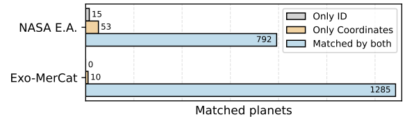
Figure 5: Yield of matched planets for the NASA Exoplanet Archive and Exo-MerCat catalogs, categorized by which methods the match was established.
