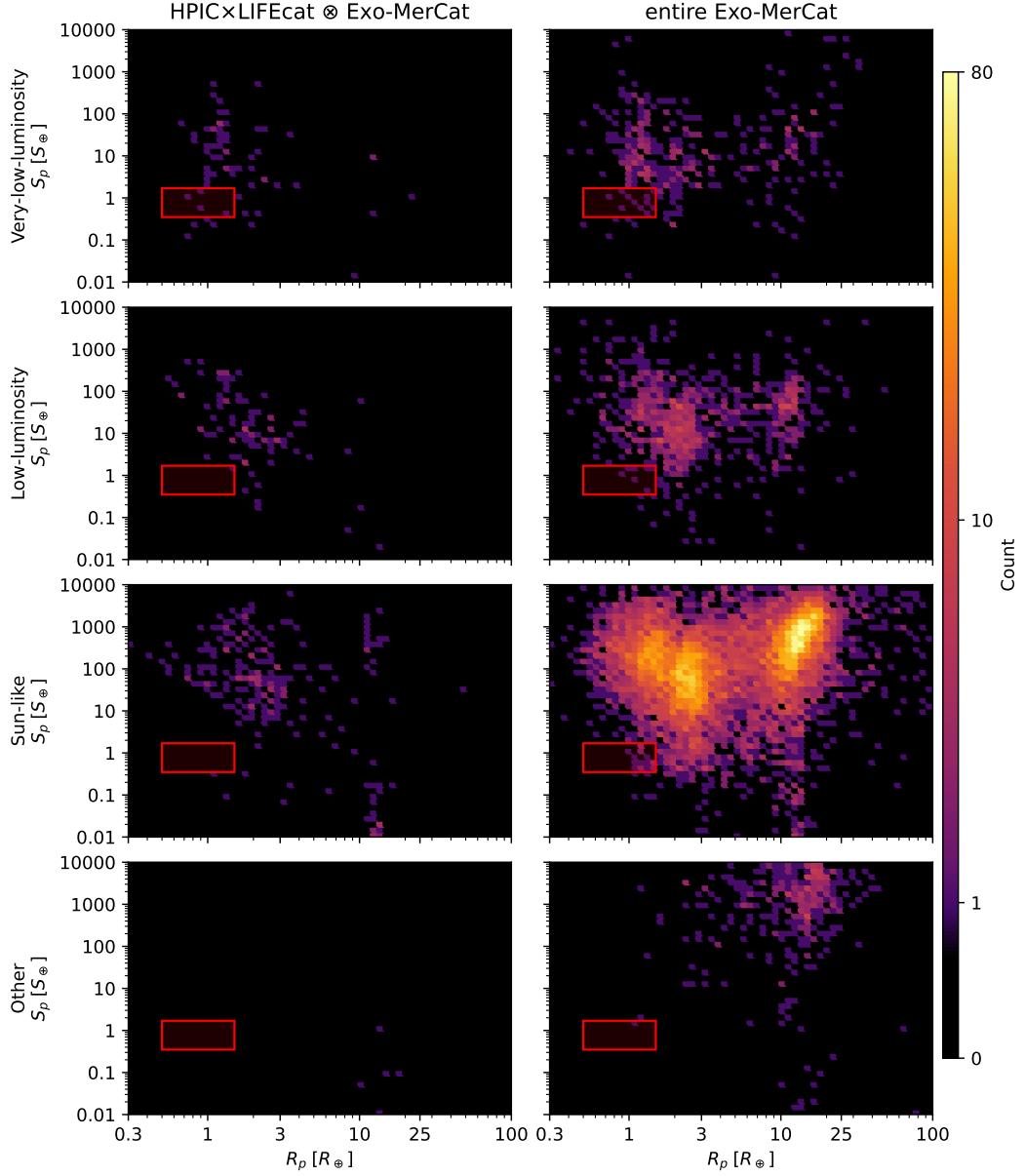
Figure 11: Two-dimensional number density of the exoplanet population in the planet-radius-insolation plane (as in figure 7), split by the spectral category of the host star. The four rows correspond to the host categories assigned by the enrichment pipeline (Very-low-luminosity, Low-luminosity, Sun-like, and Other); the left column is the distance-limited HPIC×LIFECat sample crossmatched with Exo-MerCat and the right column the entire Exo-MerCat catalog. Both axes are logarithmic and the color encodes the number of planets per bin on a logarithmic scale, shared across all panels. The red rectangle marks the rocky-and-temperate selection region ( 0.5-1.5 R_\oplus , 0.35-1.7 S_\oplus ). Planet radii and insulations are those provided by the enrichment pipeline.
