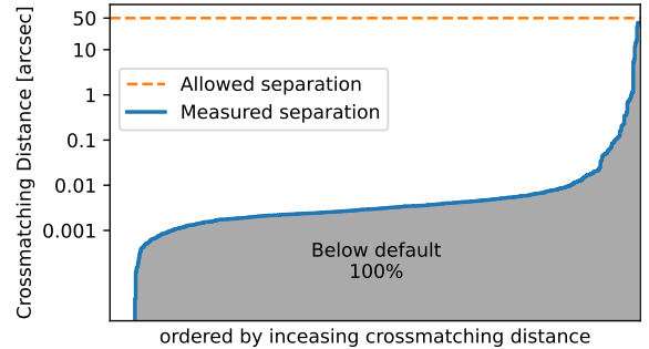
Figure 4: Calibration of coordinate crossmatching for EMC using ID crossmatches showing the measured angular separations for matched HPICxLIFECat stars with the 50” matching tolerance annotated to demonstrate that all ID-based matches remain within the adopted acceptance radius
