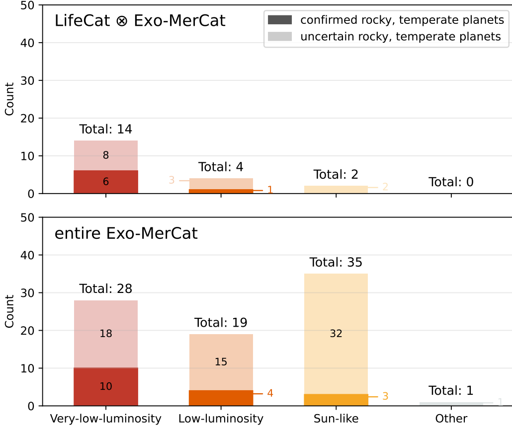
Figure 8: Yield of rocky, temperate planet candidates by host-star spectral category, using the same selection region as figure 6 and figure 7 (radius 0.5\text{--}1.5 R_{\oplus} , insolation 0.35\text{--}1.7 S_{\oplus} ). A planet is counted as confirmed (dark shading) if its central-value radius and insolation both fall inside the box and it is a confirmed planet, and as uncertain if the box is met only within the uncertainty of the radius/insolation uncertainty interval, or if the central values fall inside the box but the planet is not confirmed. The top panel shows the distance-limited HPIC \times LIFEcat sample crossmatched with Exo-MerCat (20 candidates in total), the bottom panel the entire Exo-MerCat catalog (83 candidates in total). The full list of candidates is given in Appendix section D.
