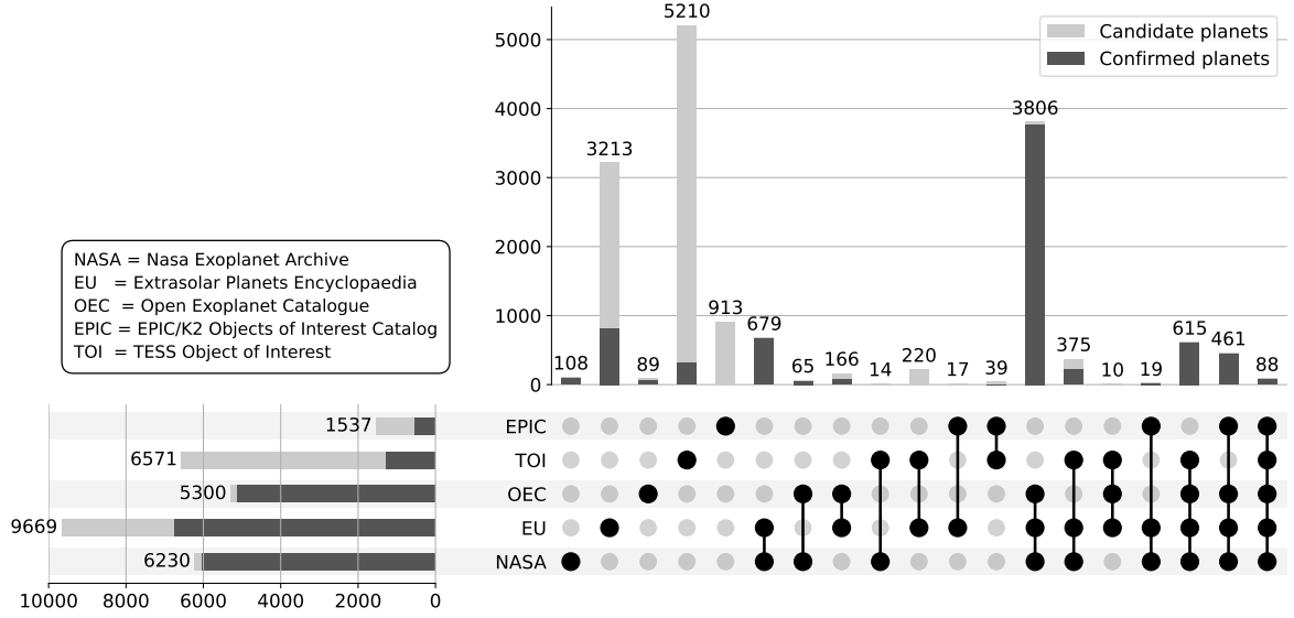
Figure 2: UpSet plot showing the overlap and distribution of exoplanets across the source catalogs of Exo-MerCat. The horizontal stacked bar chart on the left indicates the total count of planets in each catalog, while the vertical stacked bar chart at the top shows the size of the intersections of catalogs. Intersections with less than ten elements are omitted for brevity. A black dot on the line of a certain catalog means all planets in the vertical segment representing an intersection appear in that catalog. The bars are color-coded by planet status to differentiate between confirmed planets and candidate planets.
