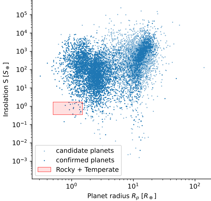
Figure 10: Distribution of the enriched Exo-MerCat exoplanet population in terms of planet-radius insolation (contains no parameter computations). Confirmed planets are drawn in the darker shade and unconfirmed candidates in the lighter shade. The red rectangle marks the rocky-and-temperate selection region adopted in this work, spanning a radius of 0.5\text{--}1.5 R_\oplus and an incident stellar flux of 0.35\text{--}1.7 S_\oplus .
