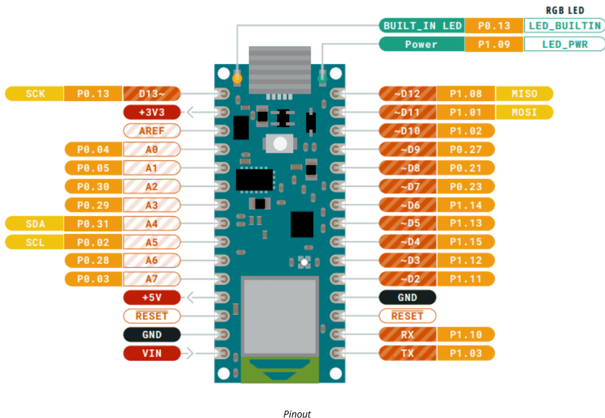
Pinout
