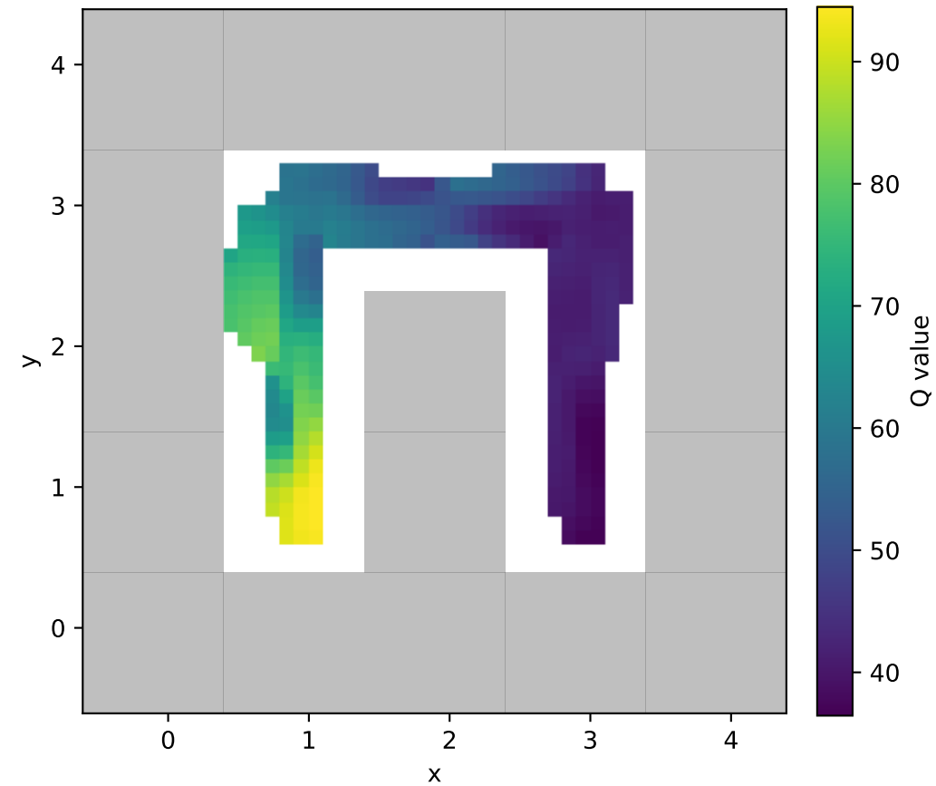
E2E\beta = 0.0
