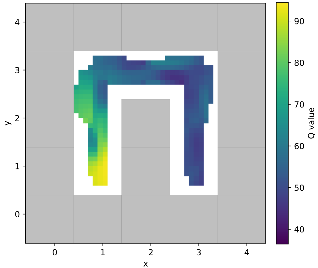
E2E\beta = 0.001
