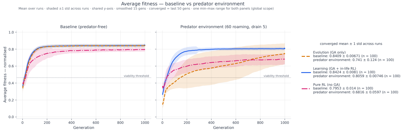
Figure 1: Normalised graph showing the mean fitness of all runs per generation for 1000 generations
