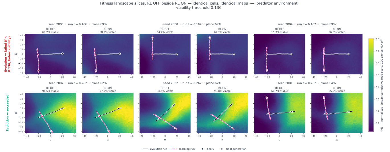
Figure 6: Fitness landscape slices of different world maps from the predator environment with a PCA trajectory of the evolution and learning runs overlaid
