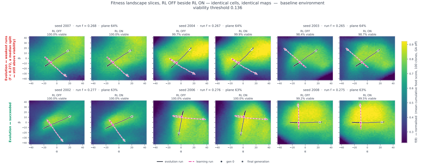
Figure 5: Fitness landscape slices of different world maps from the baseline environment with a PCA trajectory of the evolution and learning runs overlaid
