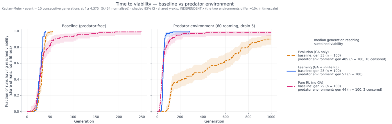
Figure 4: Graph showing after how many generations each condition crosses the viability threshold in both environments
