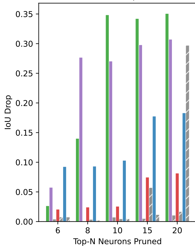
IoU Drop
