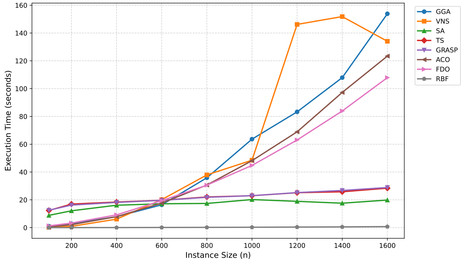
Execution Time across Instance Sizes
