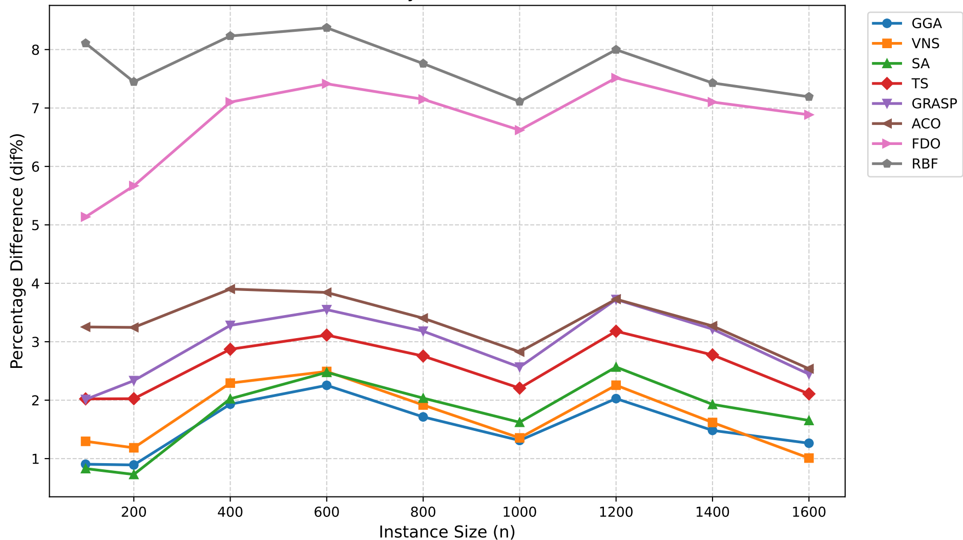
Solution Quality across Instance Sizes
