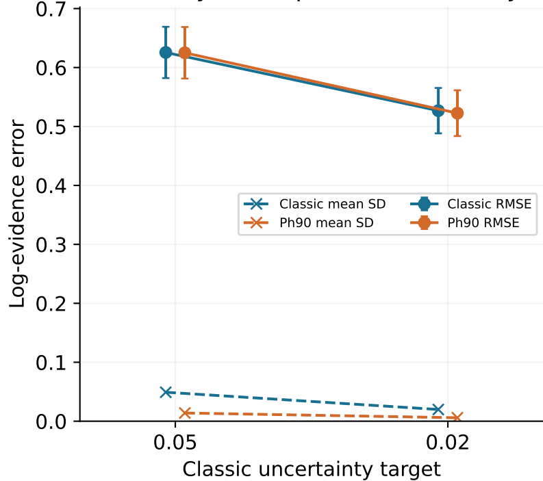
Accuracy and reported uncertainty
