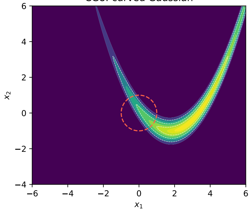
CG8: curved Gaussian
