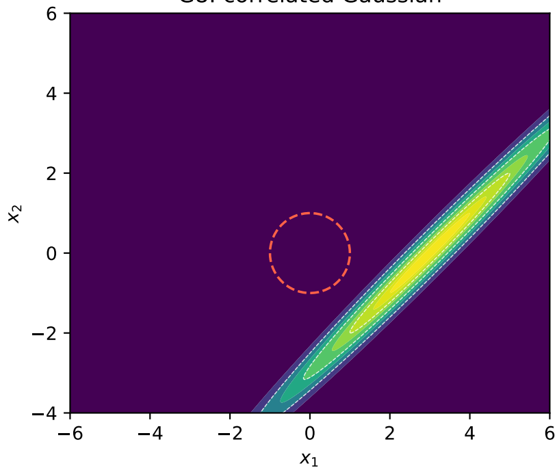
G8: correlated Gaussian
