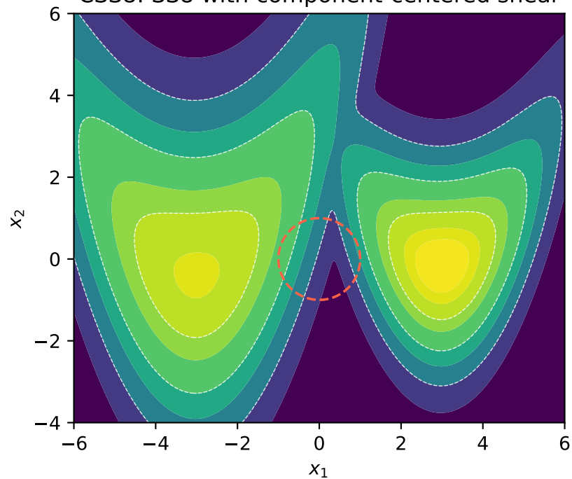
CSS8: SS8 with component-centered shear
