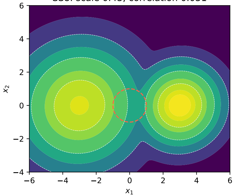
SS8: scale 0.43, correlation 0.031
