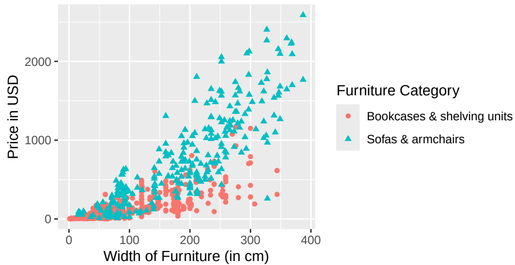
Relationship Between Price (in USD) and Width (in cm) of Ikea Furniture in April 2020
