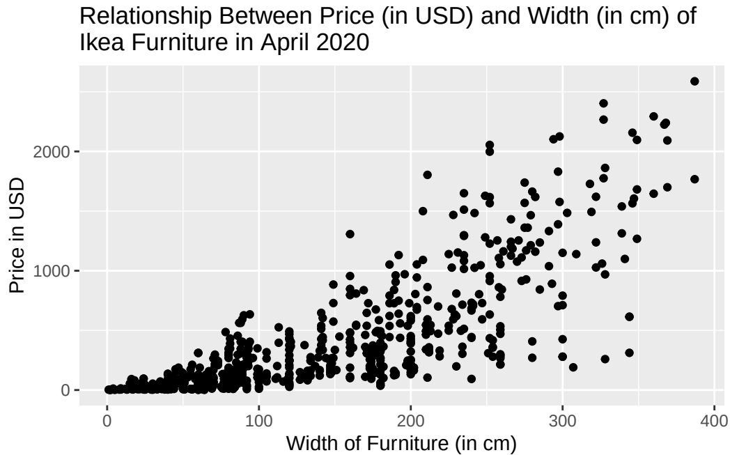
Figure 1: There is a positive nonlinear relationship between Price and Width of Ikea Furniture
