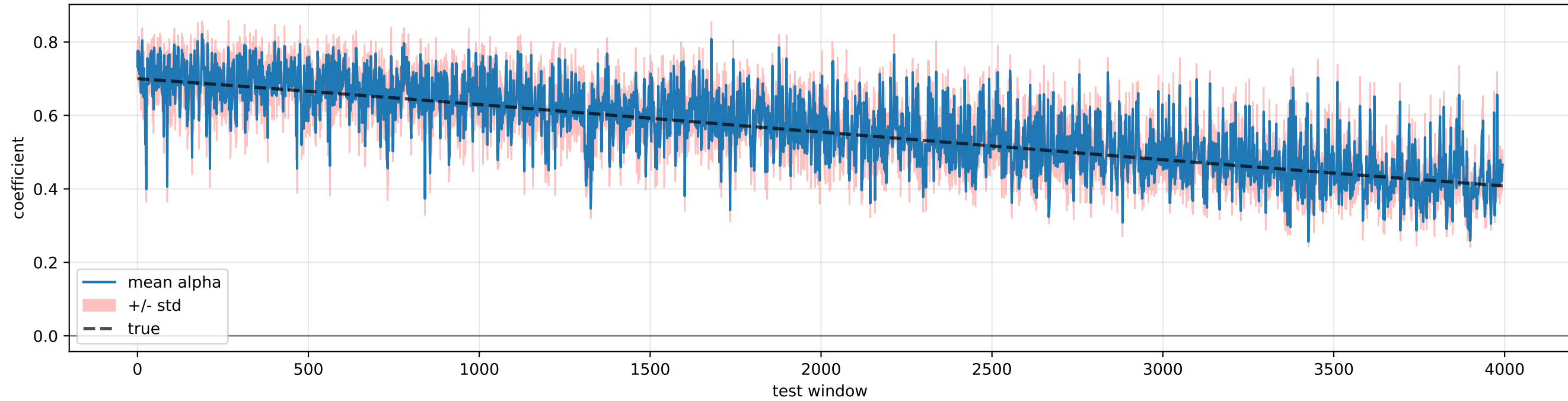
wide_mid_a0_0p10_a1_0p75_t0_0p60_s_0p30: X1 -> X2, lag 2
