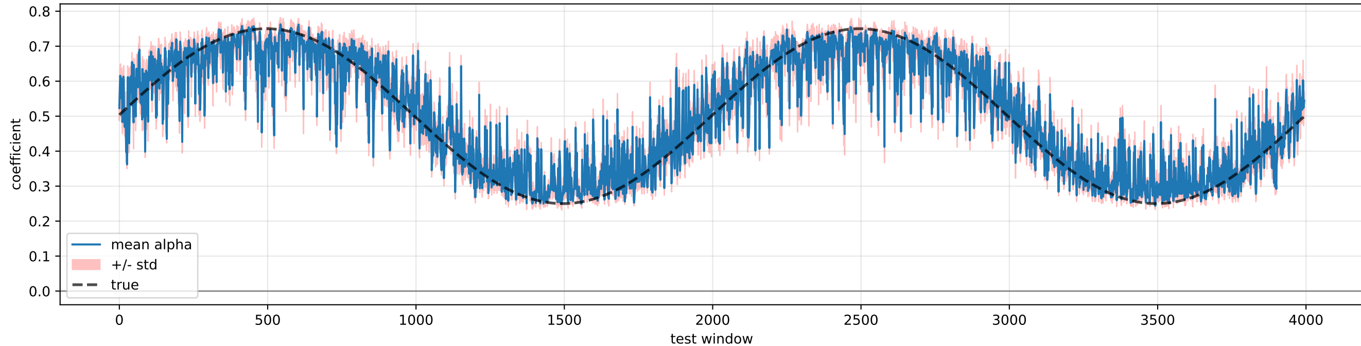
slow_period_a1_0p25_P_2000_phi_0p00: X1 -> X2, lag 2
